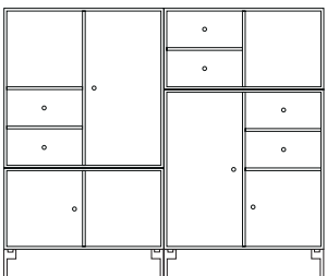
Highboard on legs W 139.2 cm H 105 cm Legs 12.6 cm
