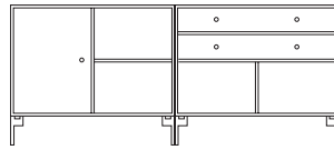
Lowboard on legs W 139.2 cm H 46.8 cm Legs 12.6 cm
