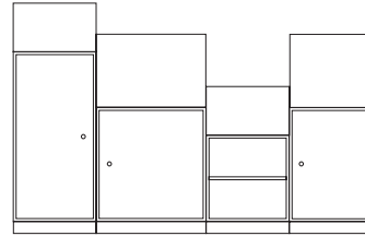
Shelving on plinth D 30 cm W 153 cm H 89.6/76.8/55.4/76.8 cm Plinth H 7 cm
