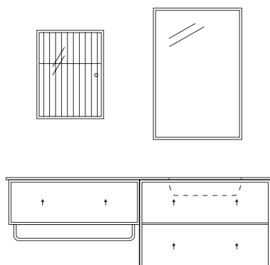
RIPPLE cabinet D 30 cm W 35.4 cm H 46.8 cm SHELFIE mirror D 9.9 cm W 46.8 cm H 69.6 cm Sink module D 48 cm W 140.8 cm H 48 cm
