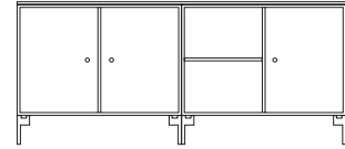
Lowboard on legs with top panel W 139.2 cm H 48 cm Legs 12.6 cm
