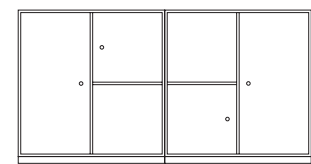
Sideboard on plinth W 139.2 cm H 69.6 cm Plinth H 3 cm
