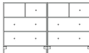
Dresser on legs W 139.2 cm H 69.6 cm Legs H 12.6 cm
