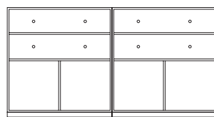
Sideboard on plinth W 139.2 cm H 69.6 cm Plinth H 3 cm
