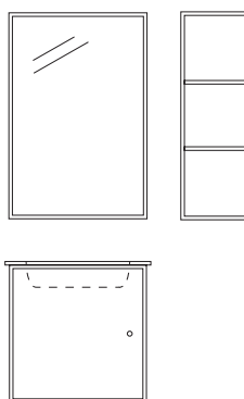
Mirror D 1.6 cm W 46.8 cm H 69.6 cm Storage module D 20 cm W 24 cm H 69.6 cm Sink module D 39.2 cm W 48.4 cm H 48 cm
