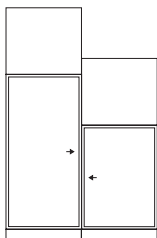
Shelving with push doors D 38 cm W 70.8 cm H 99.6/76.8 cm Plinth H 7 cm
