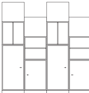
Shelving with push doors D 30 cm W 141.6 cm H 135/112.2 cm Plinth H 7 cm
