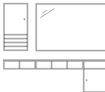
Shelving D 30 cm W 35.4 cm H 69.6 cm Mirror D 1.6 cm W 105 cm H 69.6 cm Shelving D 48 cm W 151.8 cm H 13.8/36.6 cm
