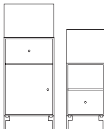
Shelving on legs D 30 cm D 30 cm W 46.8 cm W 35.4 cm H 99.6 cm H 76.8 cm Legs 12.6 cm Legs 12.6 cm
