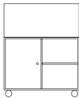
Shelving on castors D 30 cm W 69.6 cm H 76.8 cm Castors H 6.8 cm
