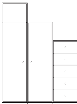
W 142.8 cm H 186.4/150.2/116 cm Plinth H 7 cm
