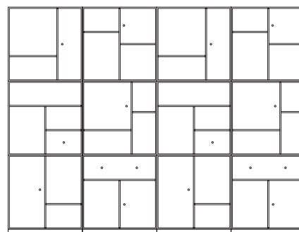
Shelving on plinth** ** W 278.4 cm H 208.8 cm Plinth 7 cm
