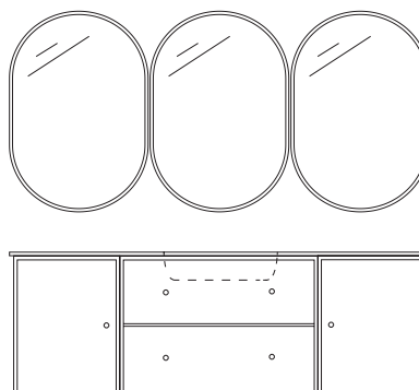
LOOK mirror x 3 D 1.6 cm W 46.8 cm H 69.6 cm Sink module D 48 cm W 142 cm H 48 cm
