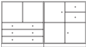
Sideboard on plinth W 139.2 cm H 69.6 cm Plinth H 7 cm
