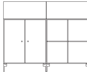
Shelving on legs D 38 cm W 139.2 cm H 99.6 cm Legs 12.6 cm
