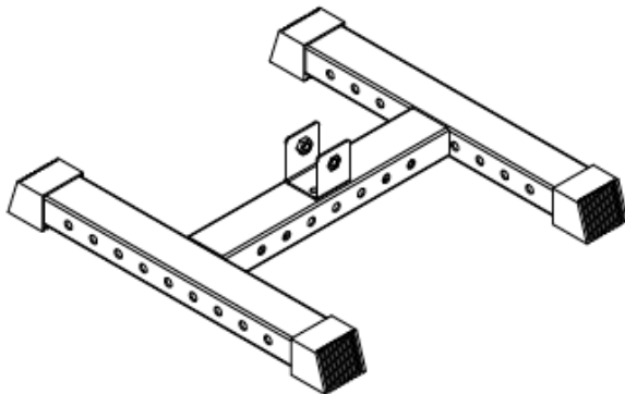
B (1) Leg base
