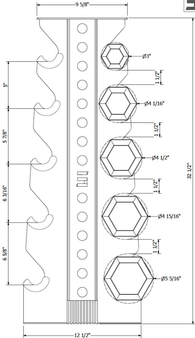
DBRK5 Bravo Vertical Dumbbell Rack | Fitting Dimensions
