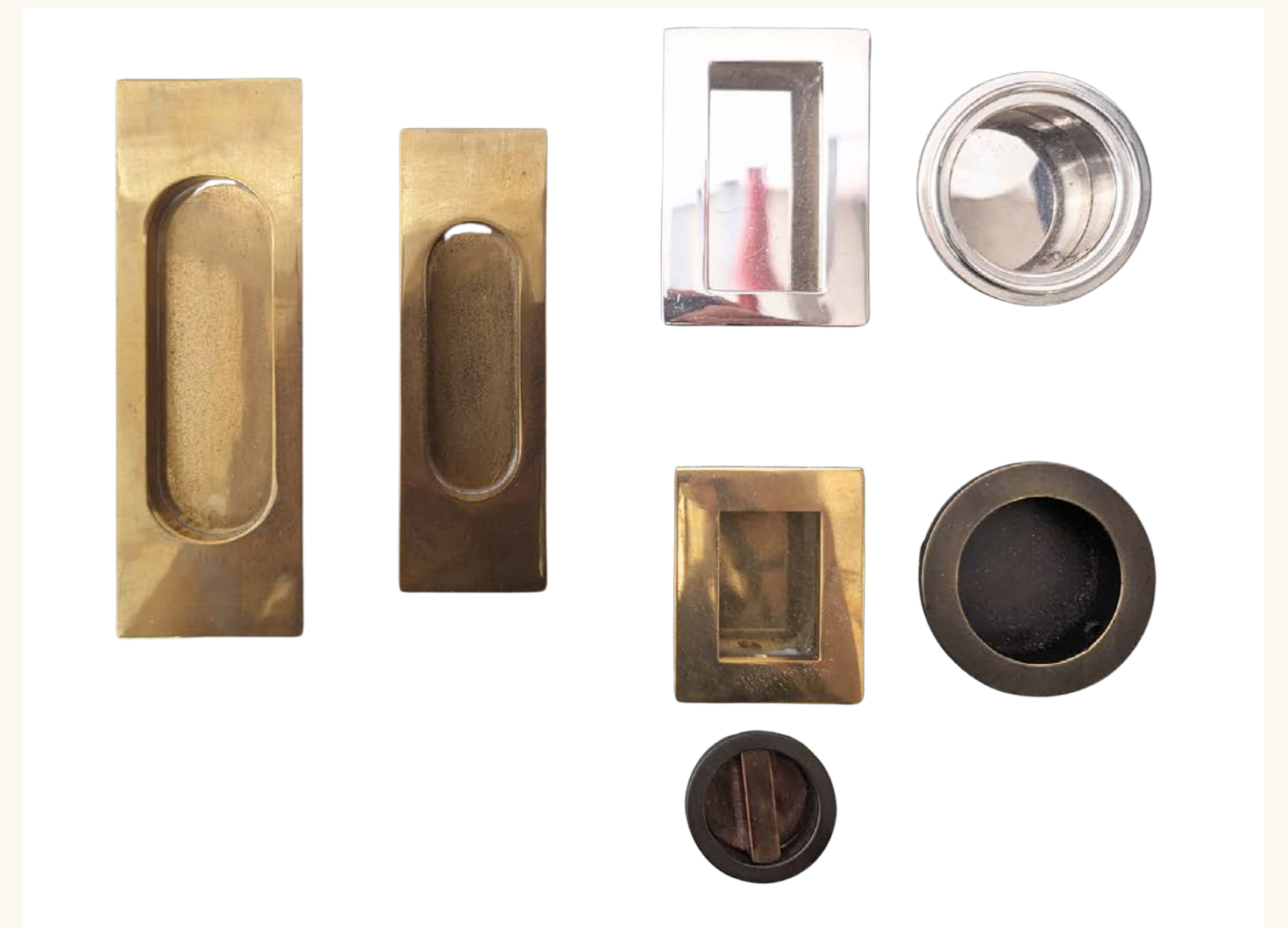
Oval flush pull - 125mm x 40mm, 150mm x 50mm, 200mm x 50mm and 300mm x 45mm - Available in a variety of finishes
