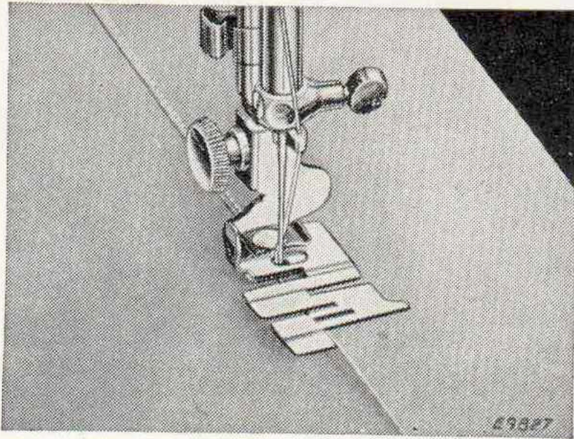
FIG. 30. MAKING A WIDE HEM.
