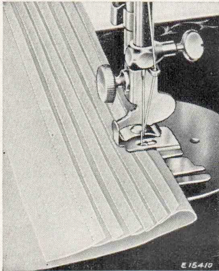
FIG. 32. TUCKING WITH THE EDGE-STITCHER.
