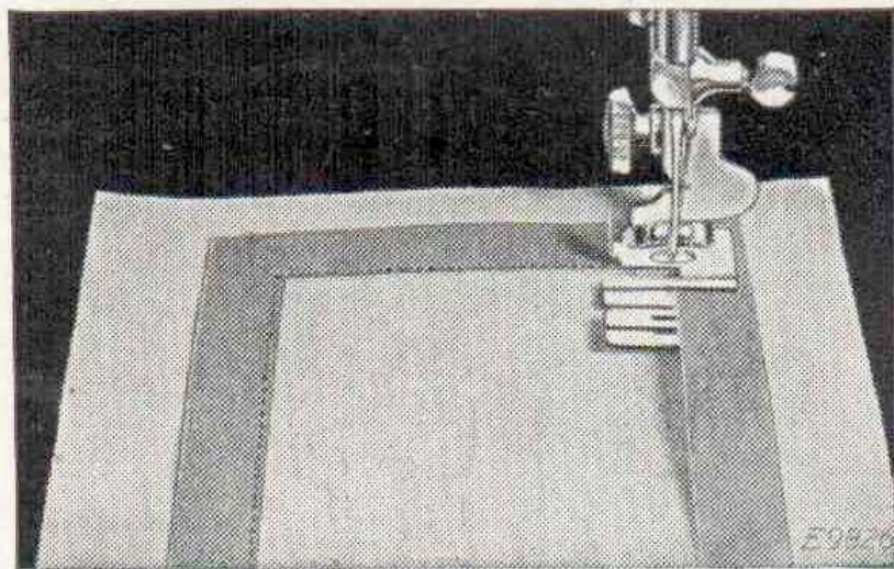
FIG. 29. APPLYING BIAS FOLDS WITH THE EDGE-STITCHER.
