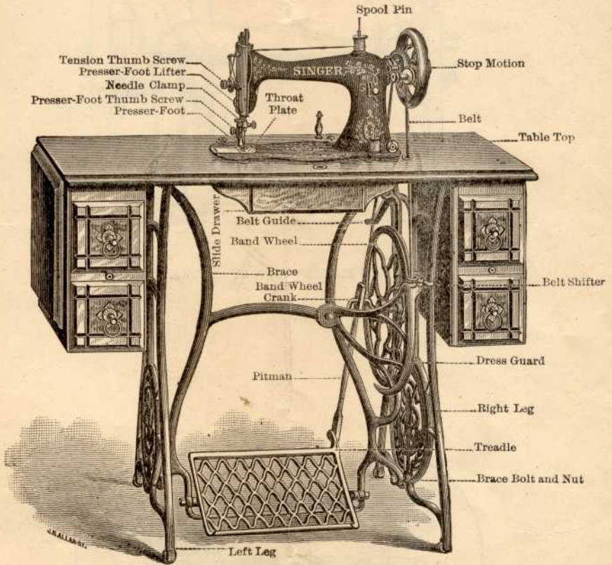
IMPROVED FAMILY MACHINE, WITH STAND.
