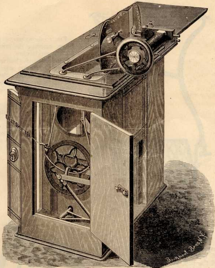
SINGER DROP CABINET (READY FOR OILING).
