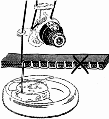
Needle thread tension too light — correct by setting dial to lower number.
