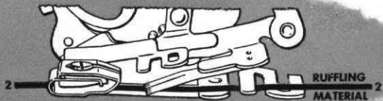
Fig. 63. Correct Position for Material to be Ruffled
