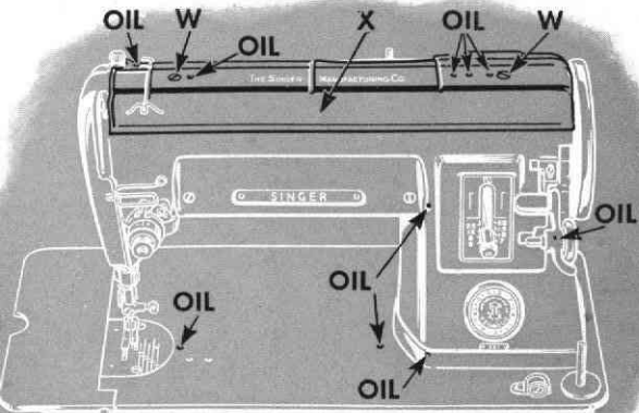
Fig. 29. Front View, Showing Oiling Points
