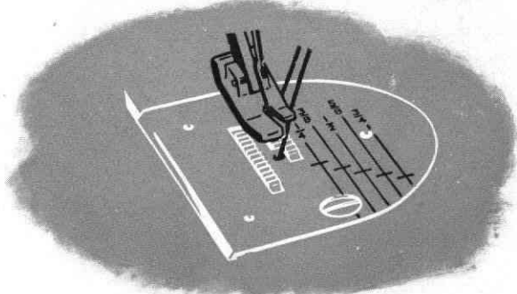
Fig. 16. Threads in Position to Start Sewing
