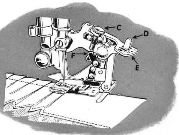
Fig. 70. Plaiting with Ruffler
