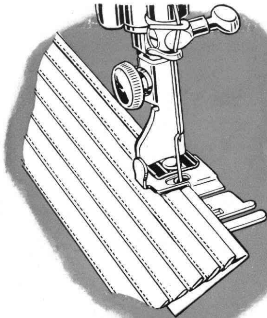
Fig. 59. Tucking with Edge Stitcher
