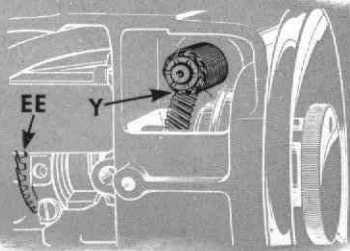
Fig. 30. Lubricating Points for Spiral Gears in Top of Machine
