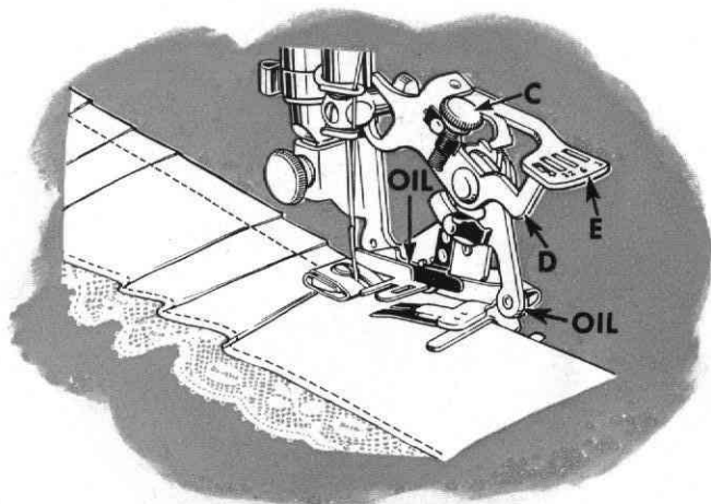
Fig. 72. Group Plaiting with Ruffler
