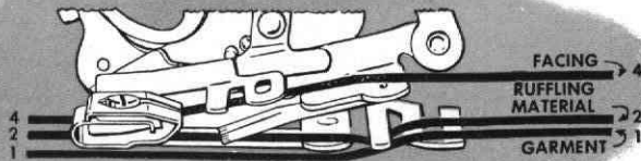
Fig. 66. Correct Positions for Materials
