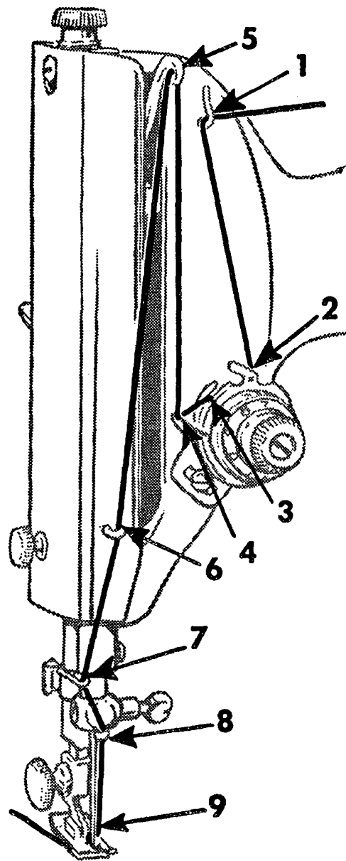
Fig. 9. Threading Tension Discs
