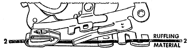
Fig. 64. Correct Position for Material to be Ruffled
