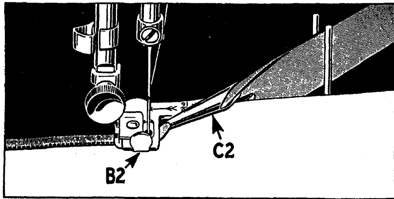
Fig. 49. Binding with Unfolded Binding
