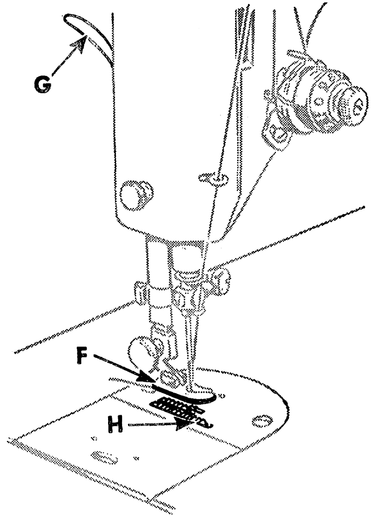
Fig. 7. Front View of Machine
