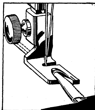
Fig. 44. Making a Felled Seam (Second Operation)
