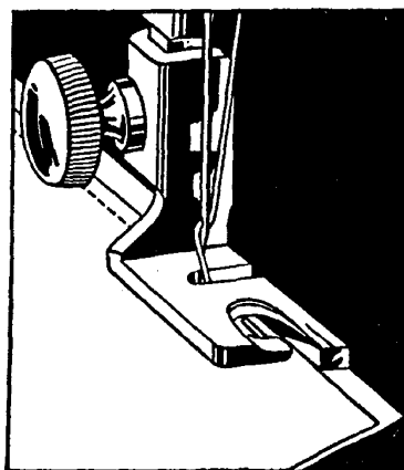
Fig. 43. Making a Felled Seam (First Operation)
