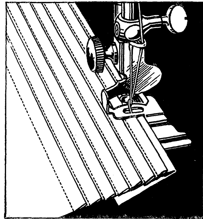
Fig. 61. Tucking with Edge-Stitcher
