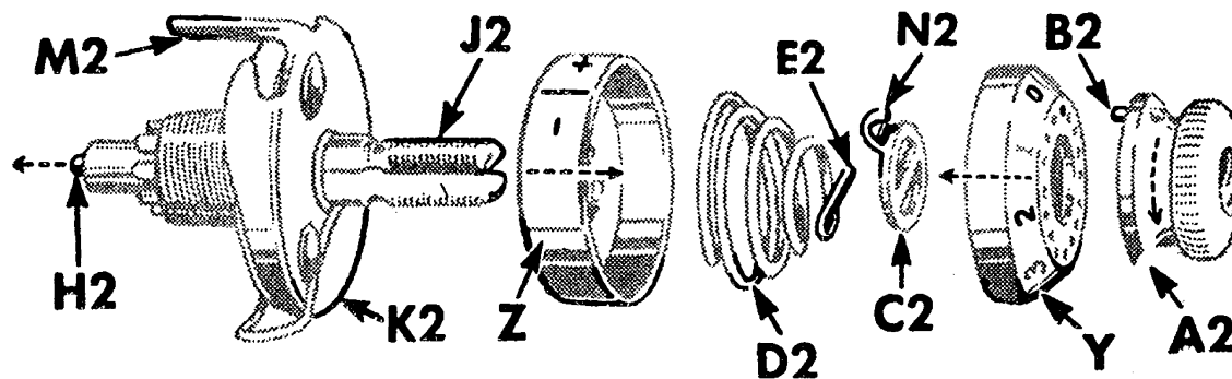
Fig. 27. Needle Thread Tension Disassembled
