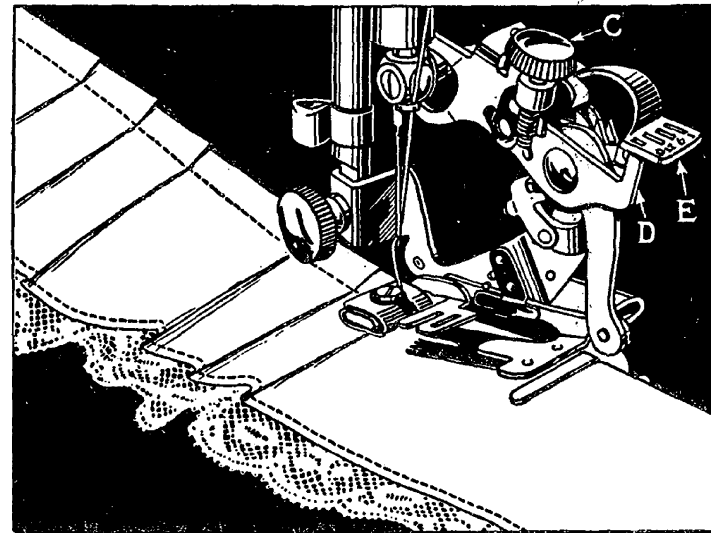
Fig. 74. Group Pleating with Ruffler
