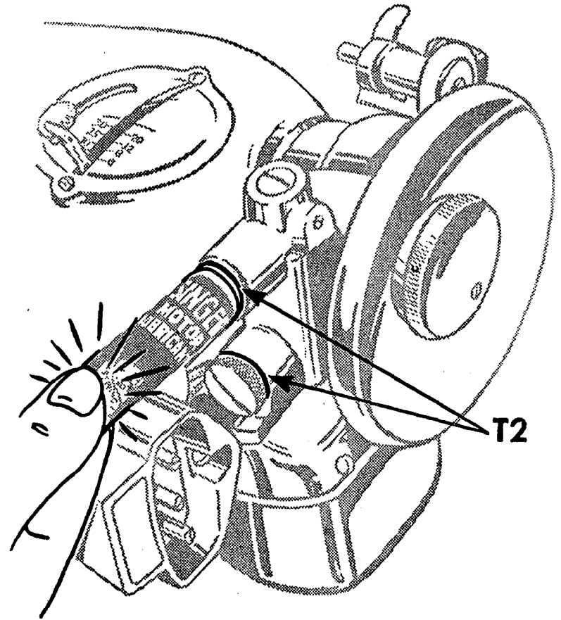
Fig. 35. Lubricating the Motor
