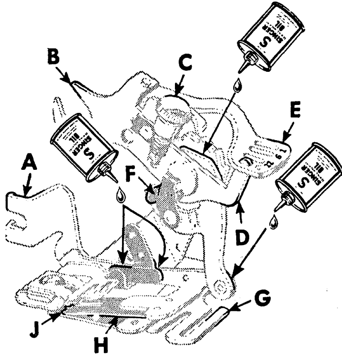
Fig. 63. Principal Parts of Ruffler
