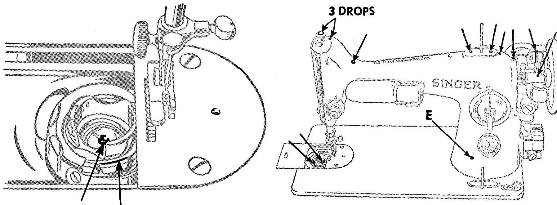
Fig. 31. Front Views Showing Oiling Points
