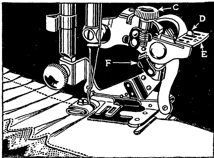
Fig. 73. Pleating with the Ruffler
