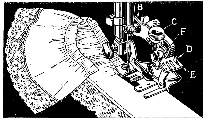
Fig. 65. Gathering with Ruffler
