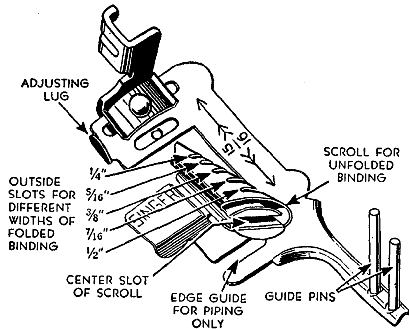
Fig. 47. Multi-Slotted Binder 160359
