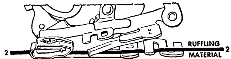
Fig. 72. Correct Position for Material
