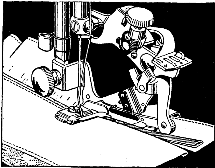
Fig. 71. Piping a Ruffle
