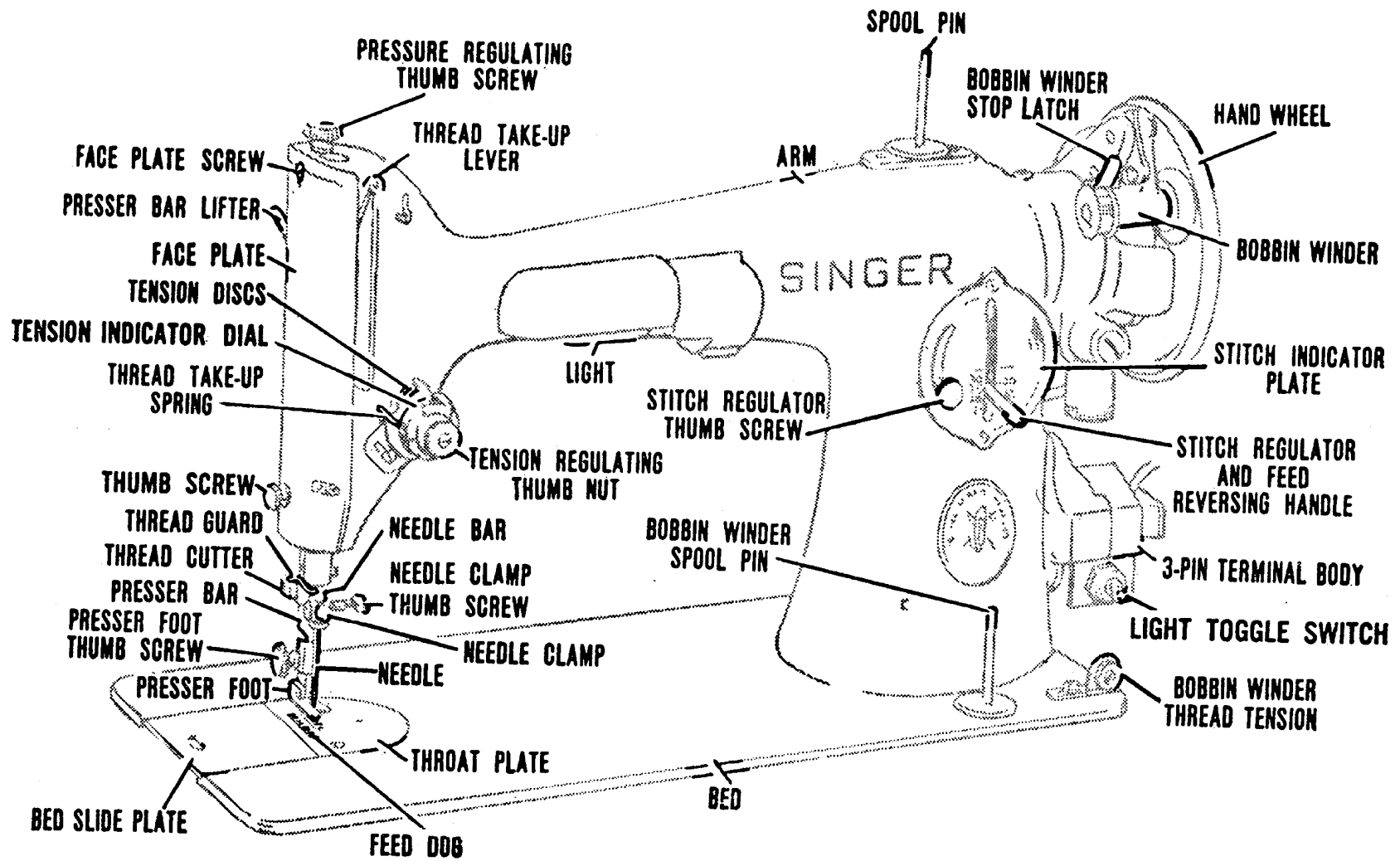
Fig. 2. Names of Principal Parts of Machine
