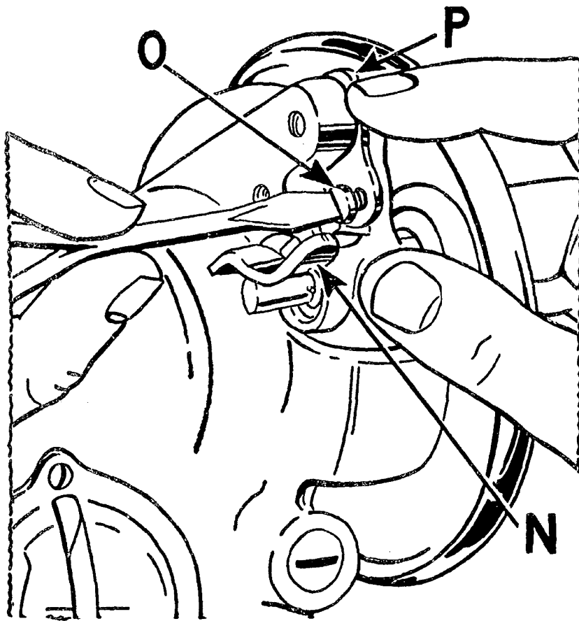
Fig. 12. Adjustment of Bobbin Winder
