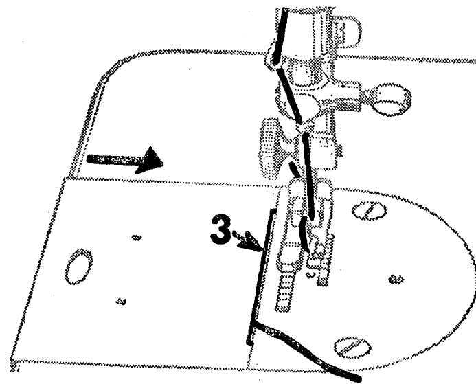
Fig. 16. Under Threading Completed
