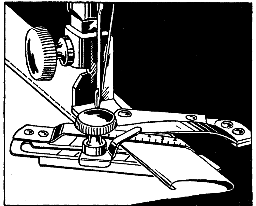
Fig 46. Making Hem Up to \frac{15}{16} Inch Wide With Adjustable Hemmer
