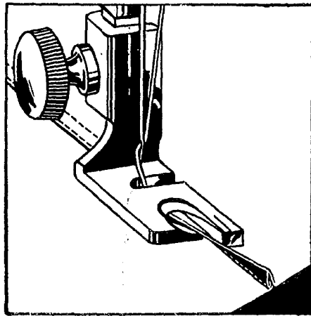
Fig. 42. Making a Hemmed Seam (Second Operation)
