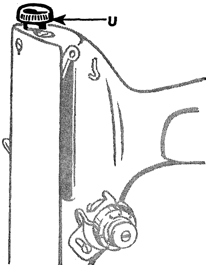
Fig. 22. Thumb Screw for Adjusting Pressure
