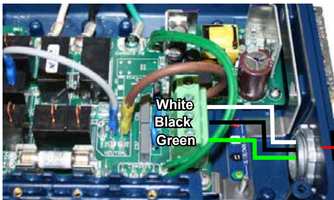
Field Converted 115V 30 Amp Control Box
