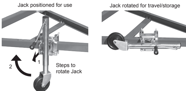
Figure C: Jack Positions
