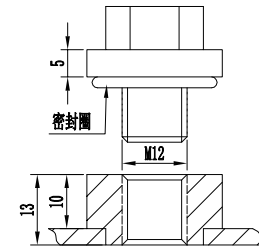
Air(Oil) release plug
