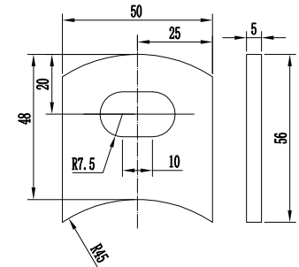
Fixing plate
