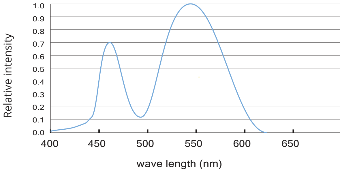
Ribbon Series LED Strip with 2835 SMD LEDs (60 LEDs/meter) Photoelectric Parameters: 12VDC power; 13.2W±10%
