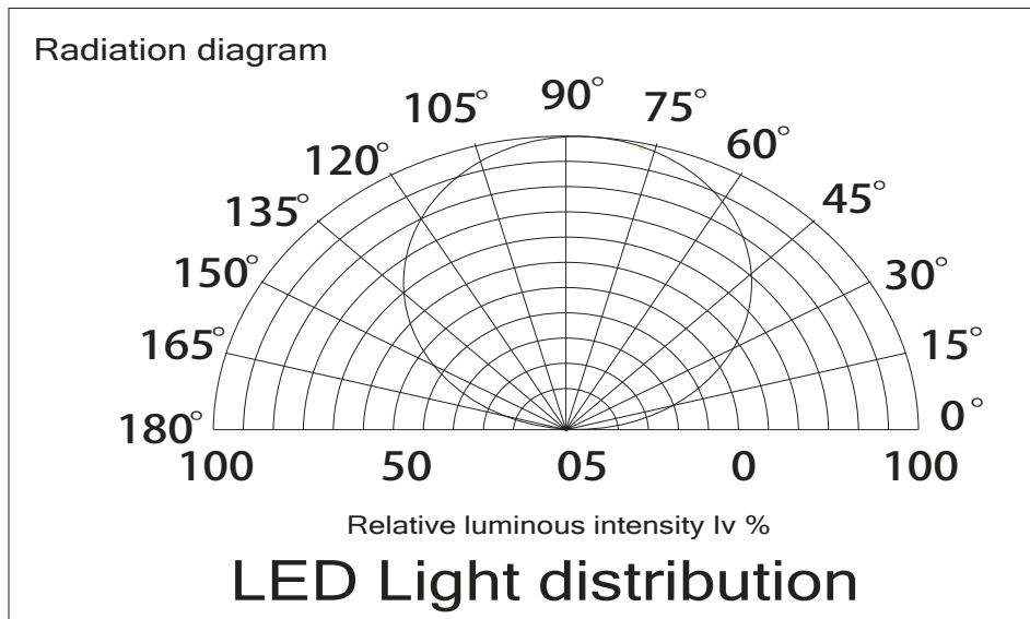
Ribbon Series LED Strip with 2835 SMD LEDs (60 LEDs/meter) Photoelectric Parameters: 12VDC power; 13.2W±10%
