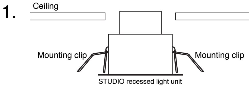
Mounting clips
