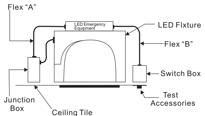
Illustration 1 Downlight Fixture
