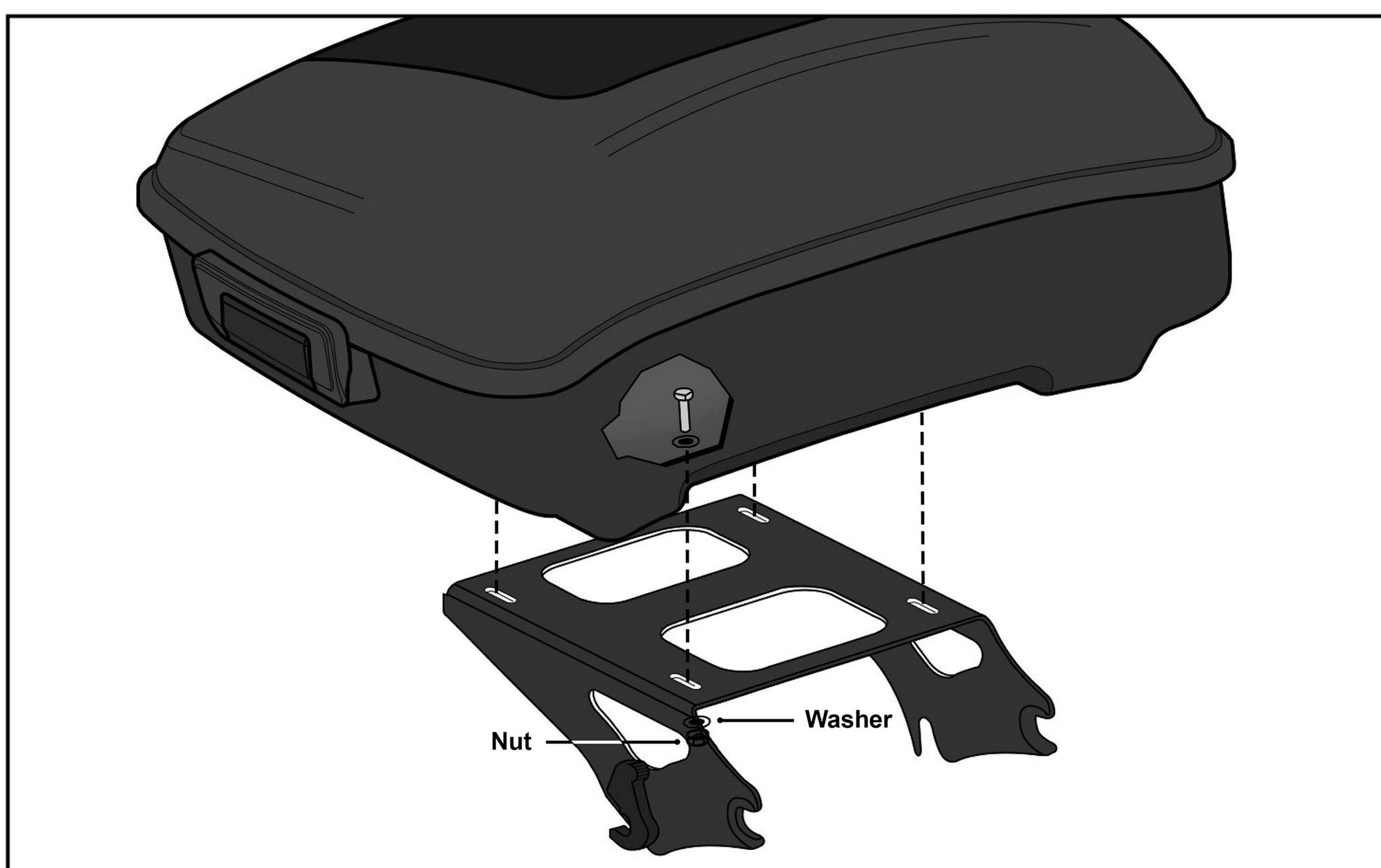
(Figure 1). Mounting the Tour Pack
