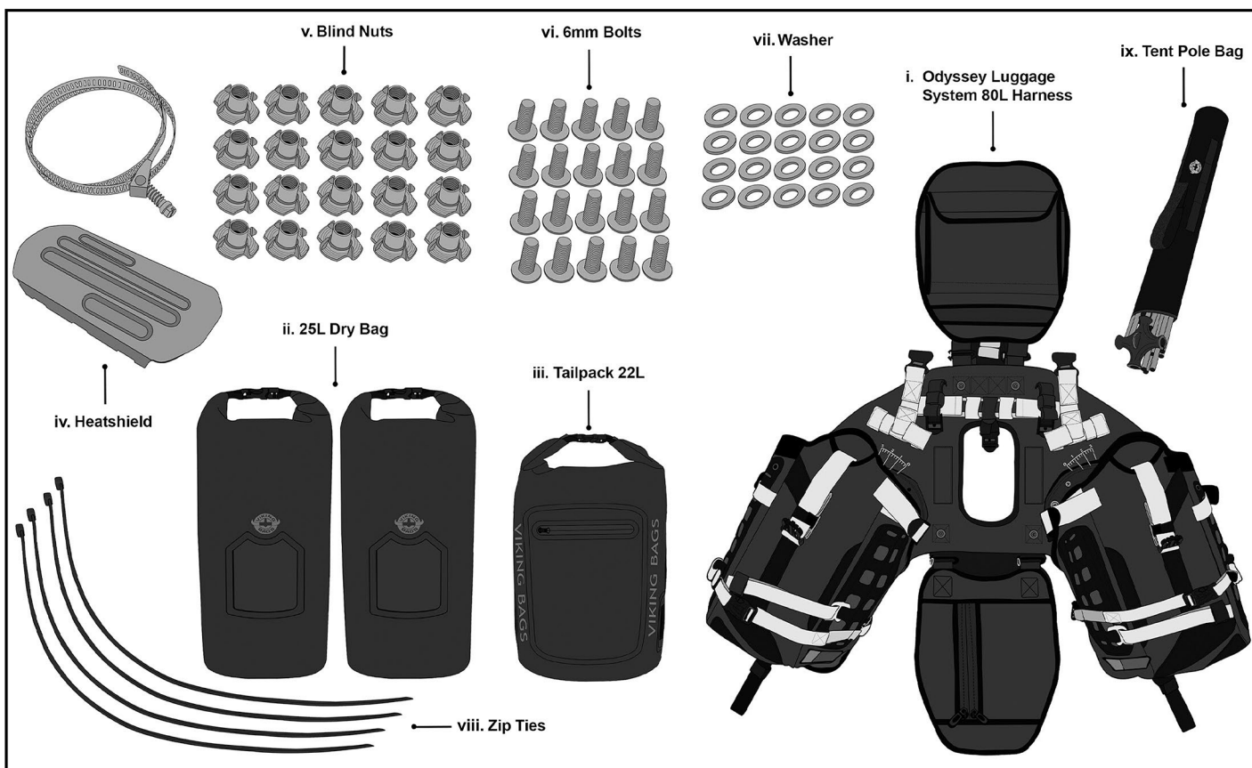
Fig 1. Parts List
