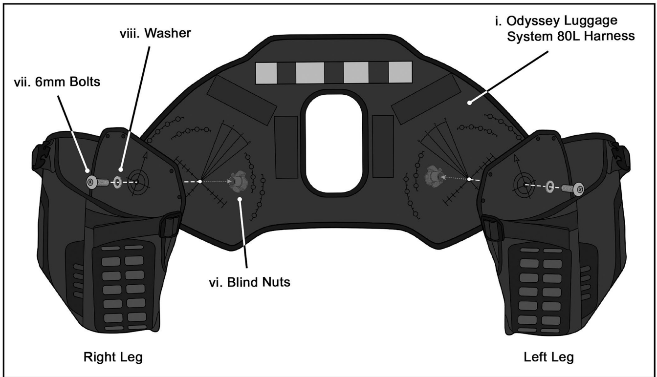
Fig 1. Attaching the legs to the harness
