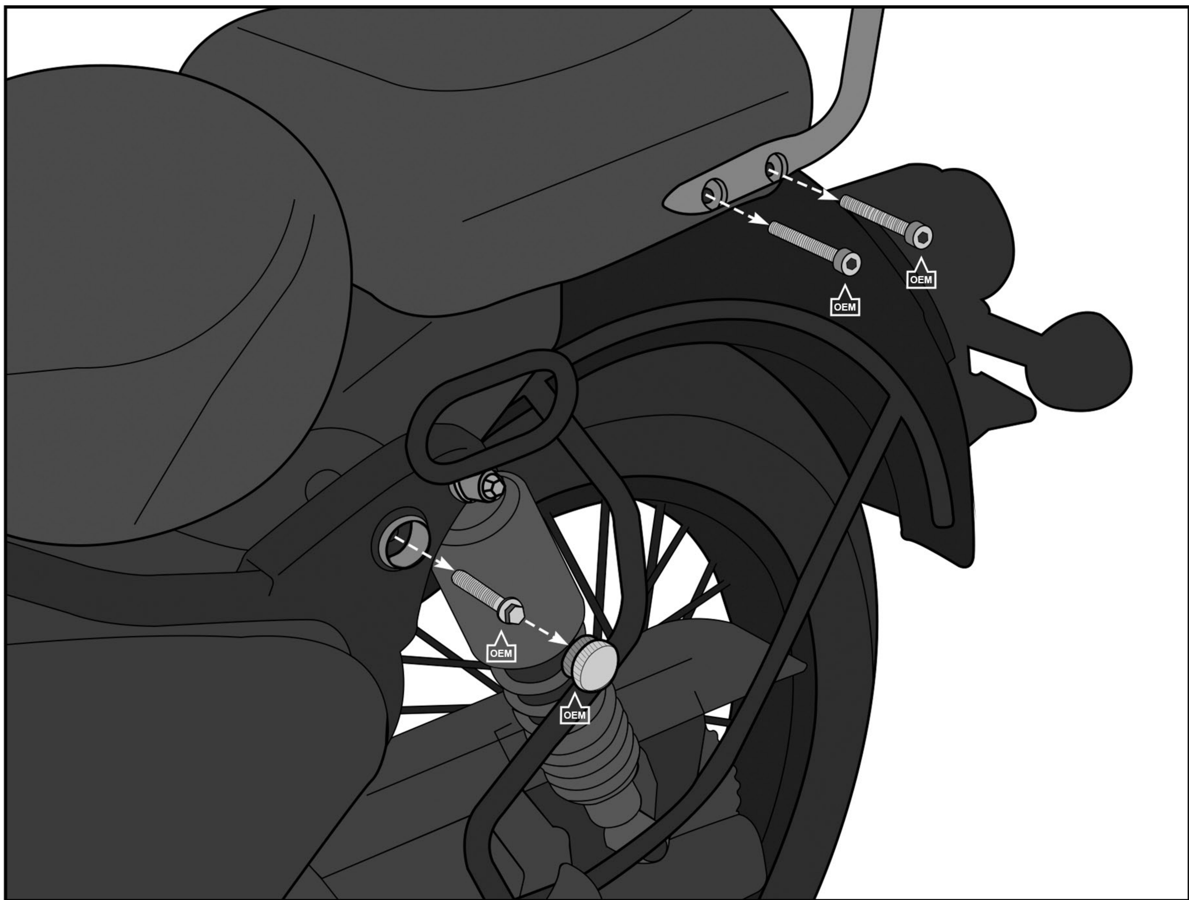
Fig 1. Remove OEM bolts
