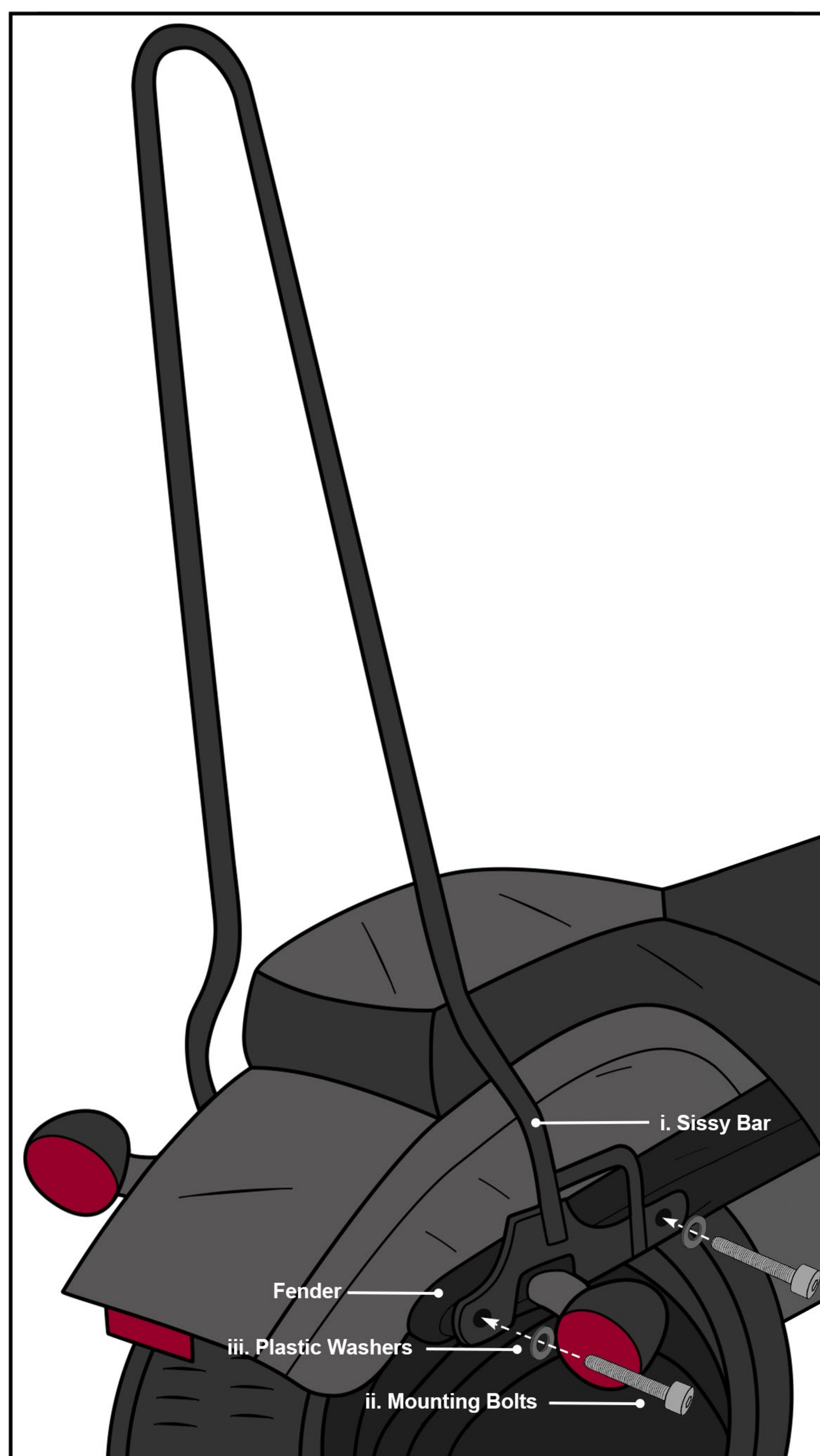
(Fig A) Sissy Bar Installed on Sportster
