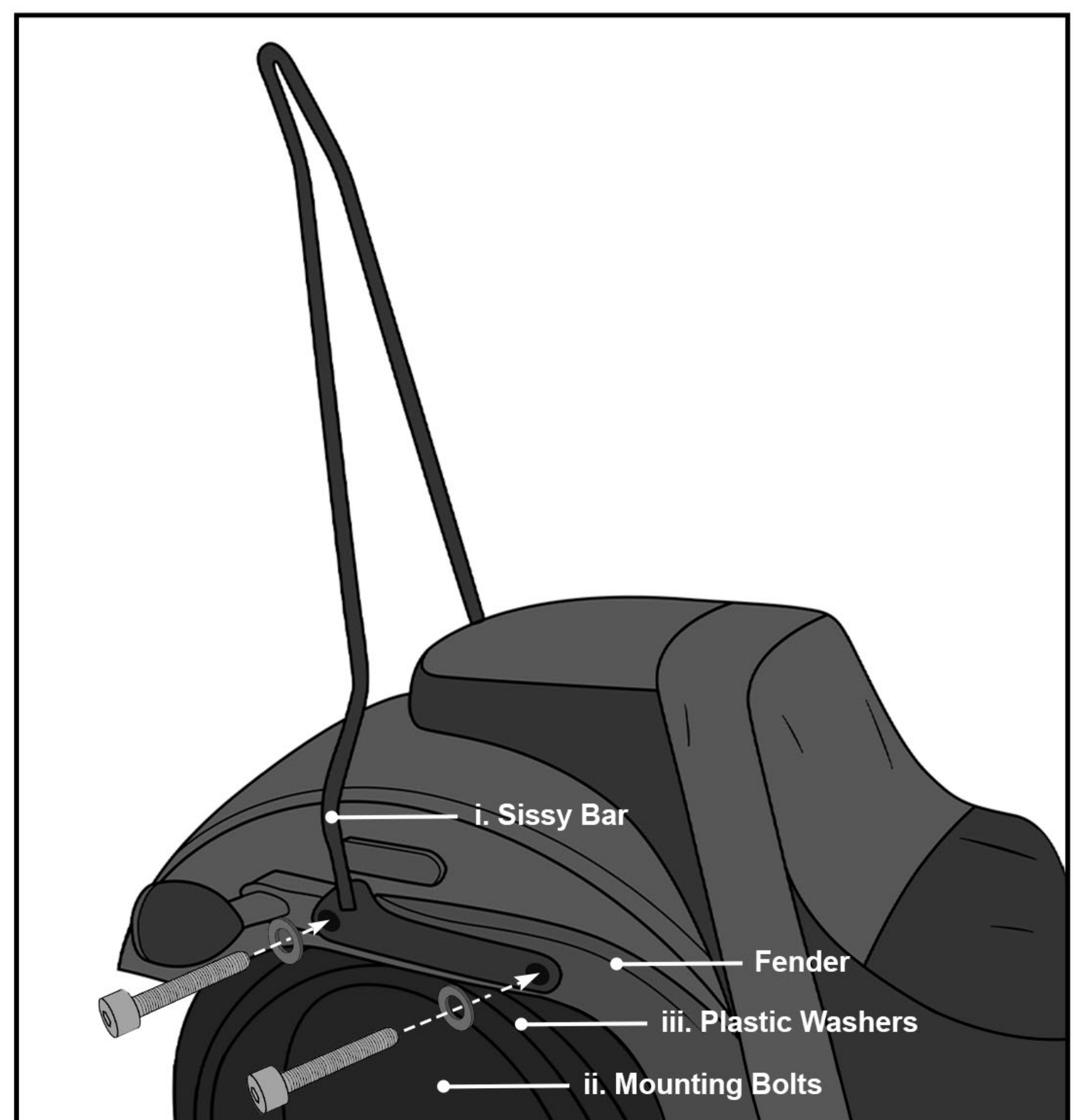
(Fig A) Sissy Bar Installed on Sportster
