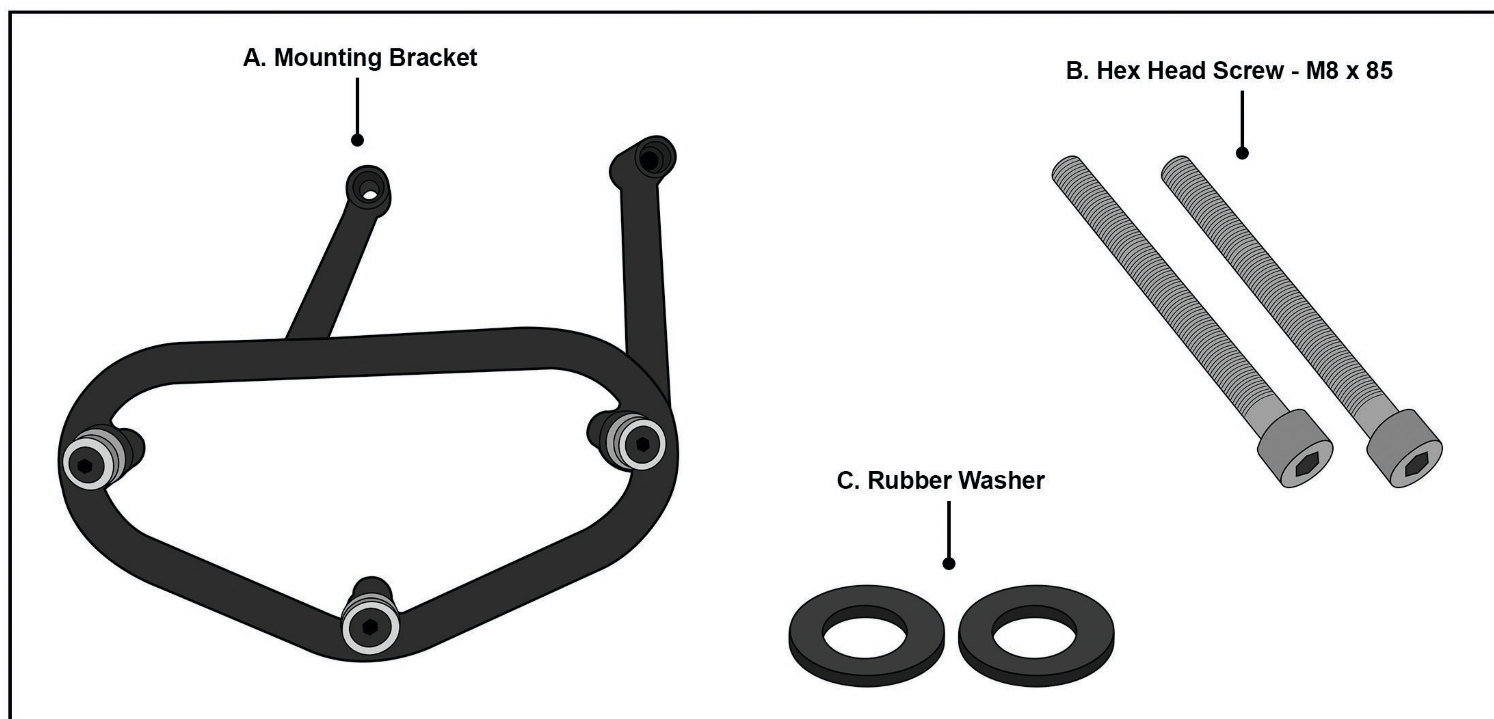
Parts Diagram
