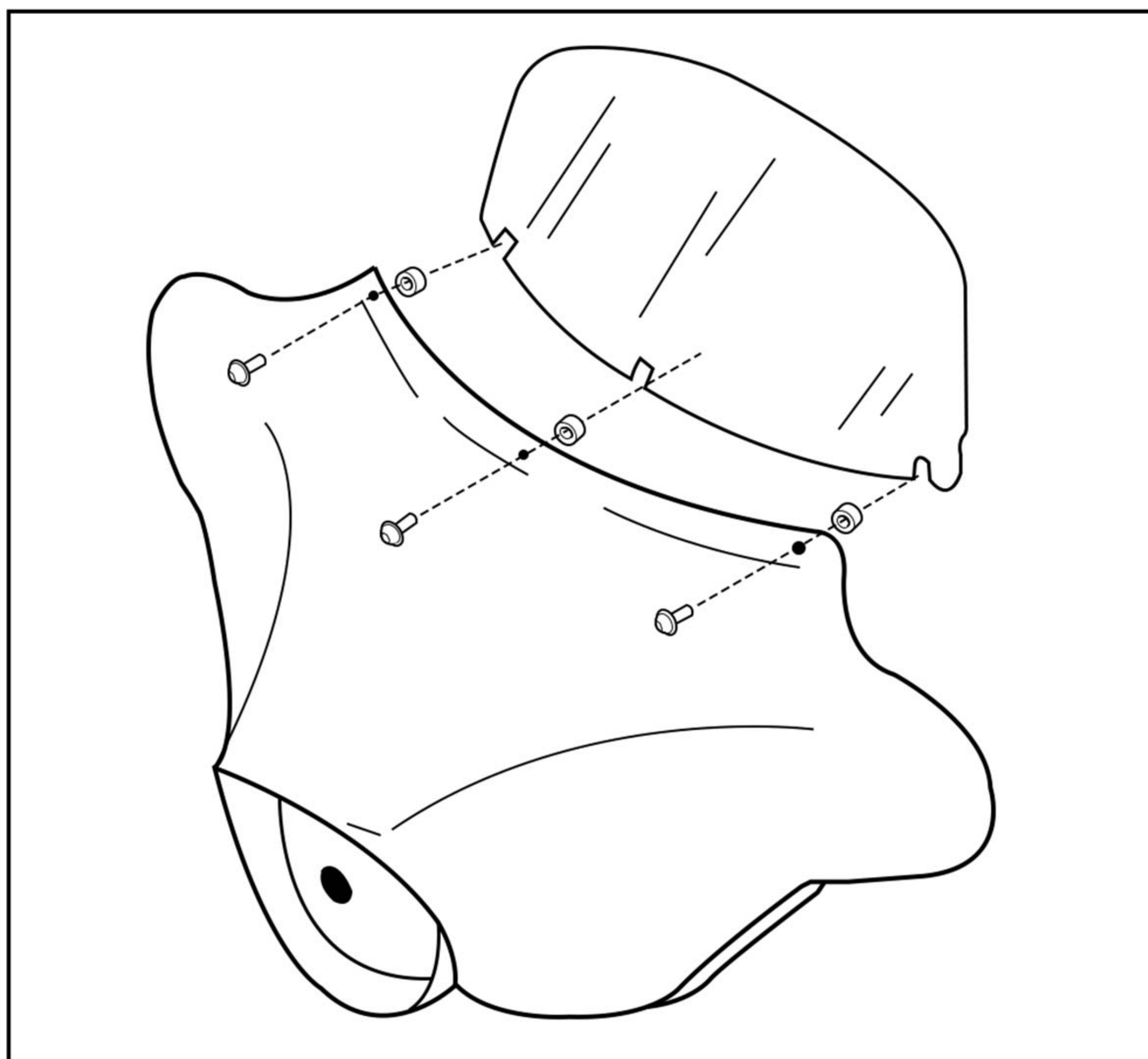
Figure 2. Install the three mounting screws and spacers.
