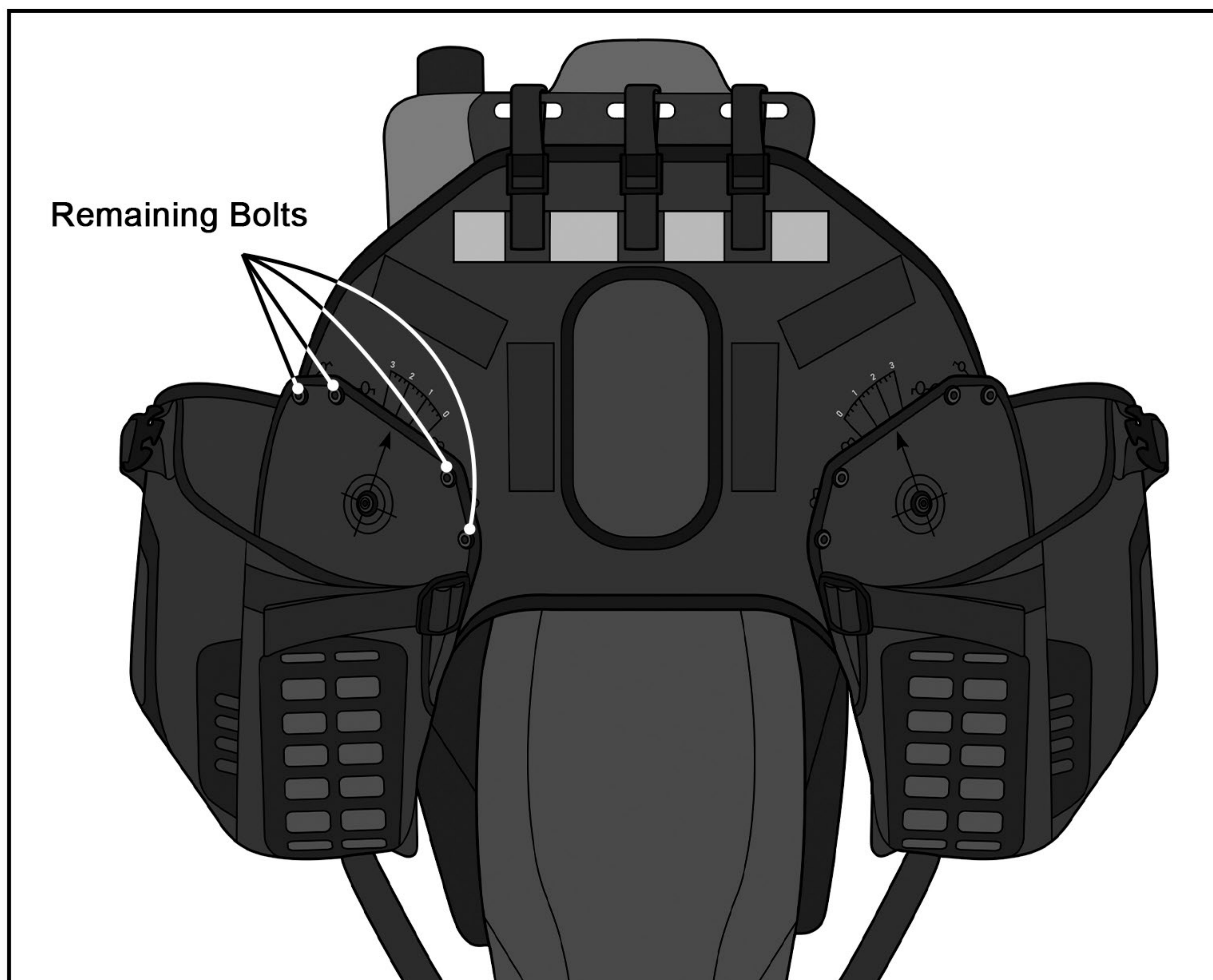
Fig 3. Installing the remaining bolts
