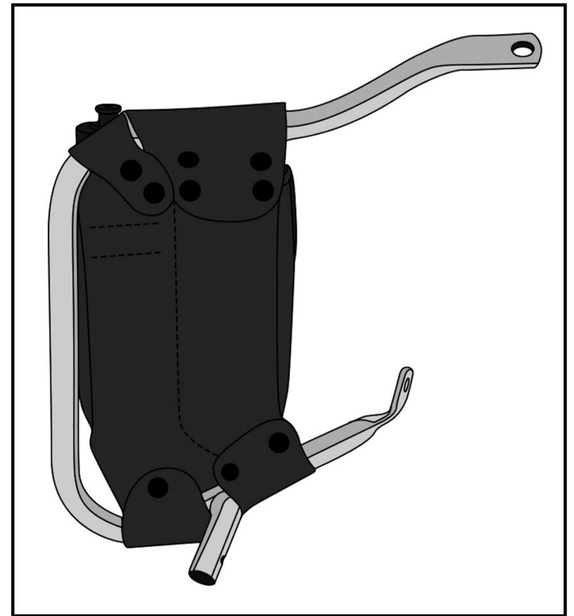
Fig (A). Install the bag on saddlebag guard, using snap set.
