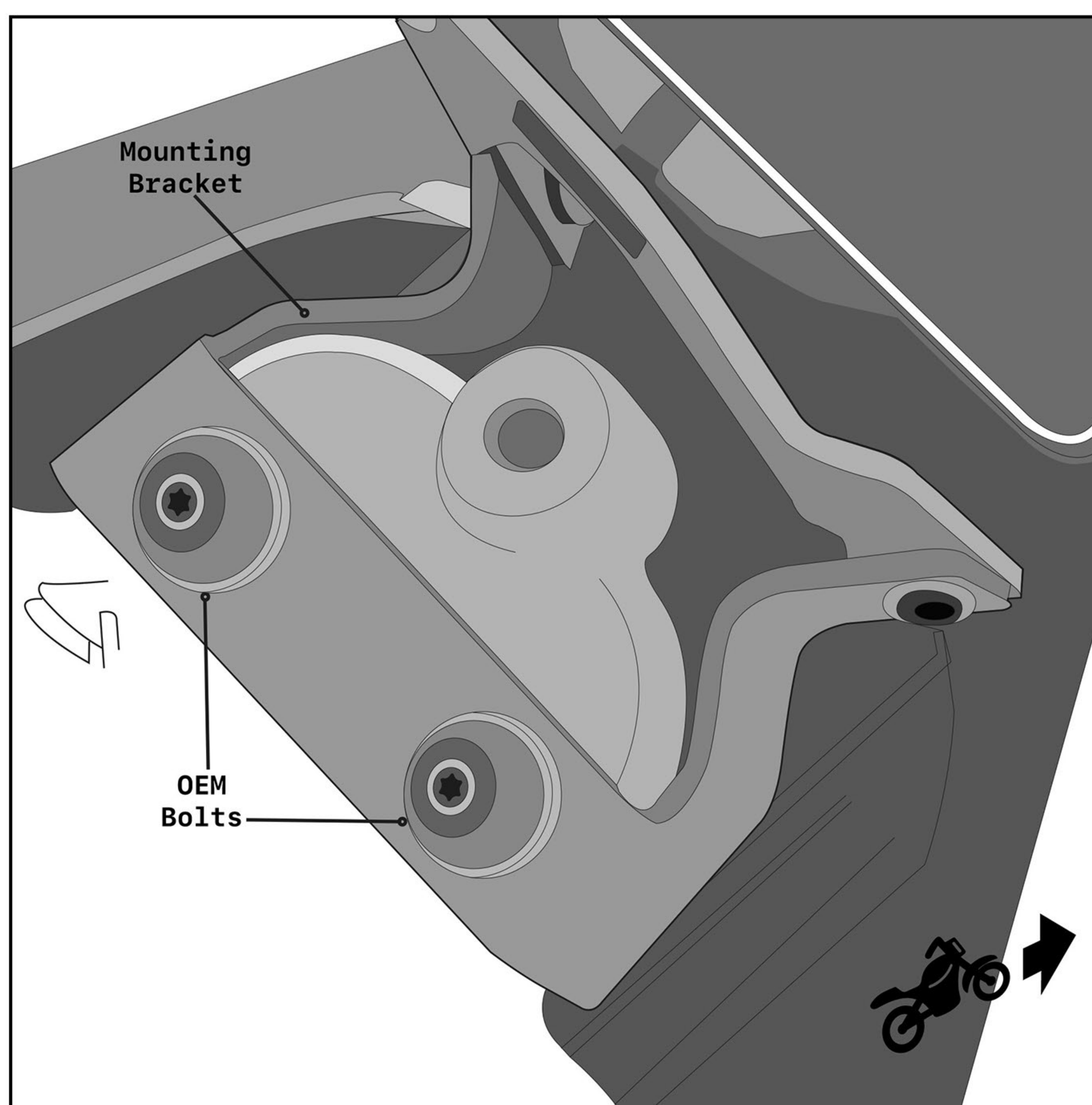
(Fig 2) Installation of Mounting Bracket
