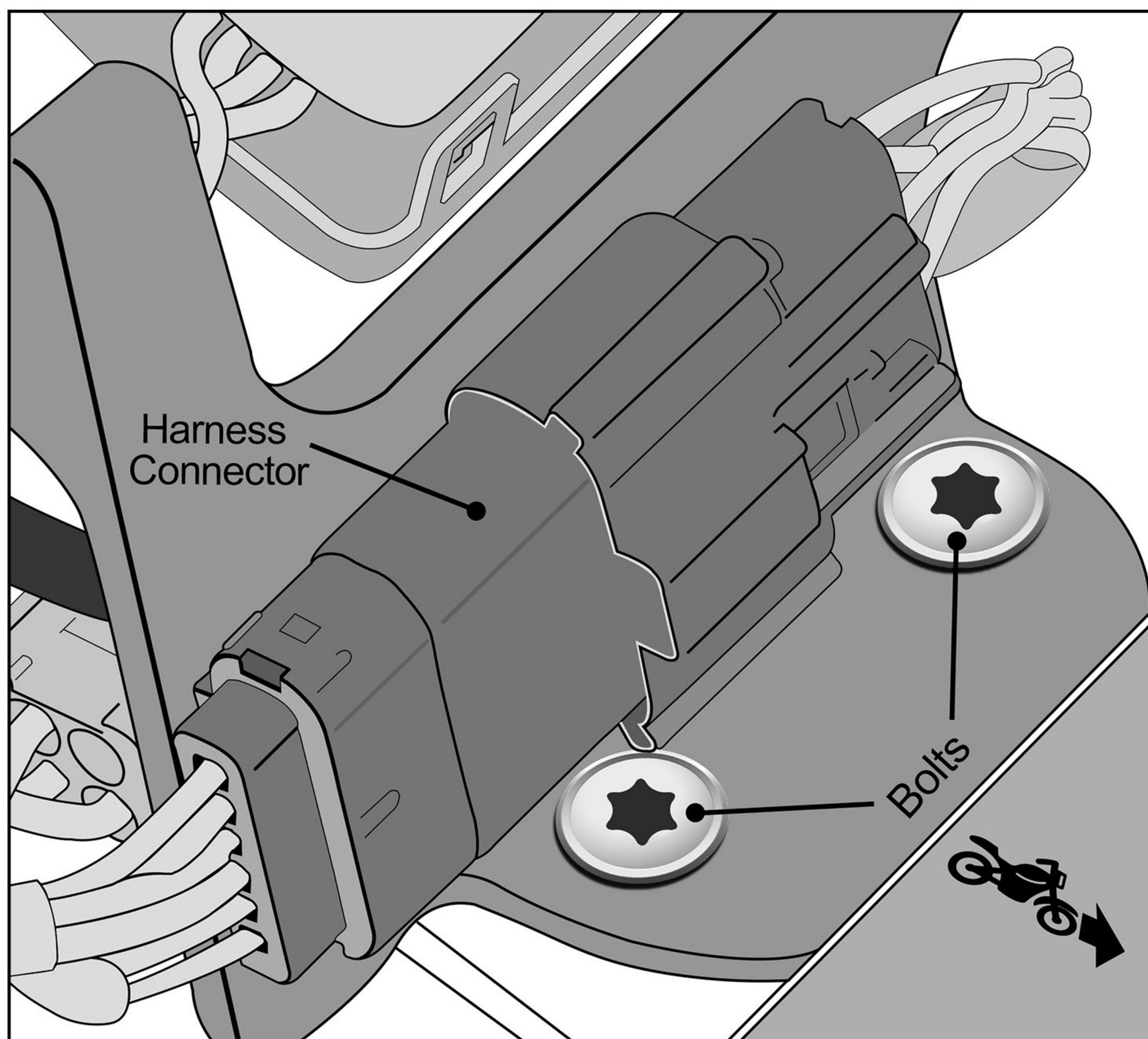
(Fig 1) Gain access to the screws by moving the harness connector away from the carrier caddy
