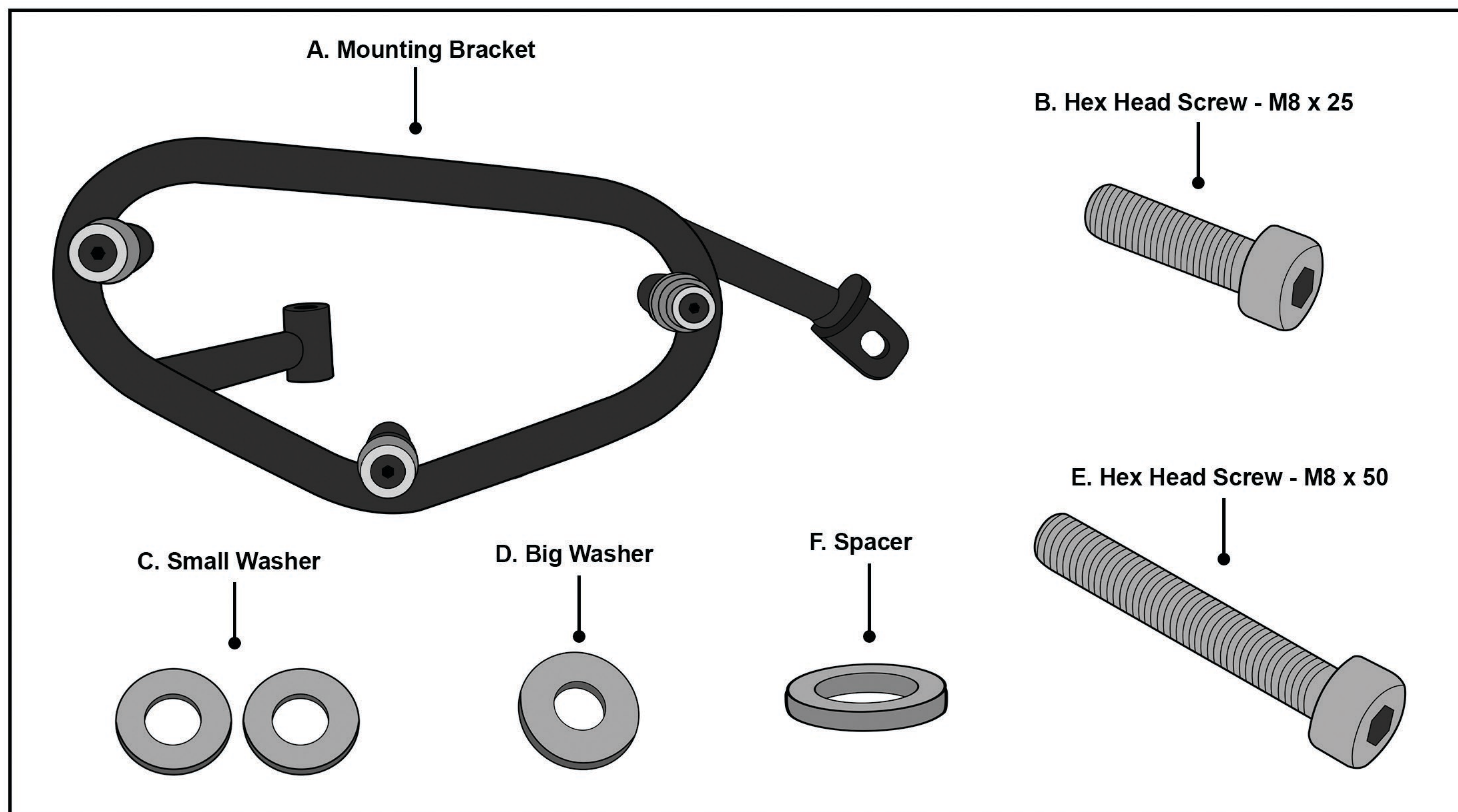
Parts Diagram
