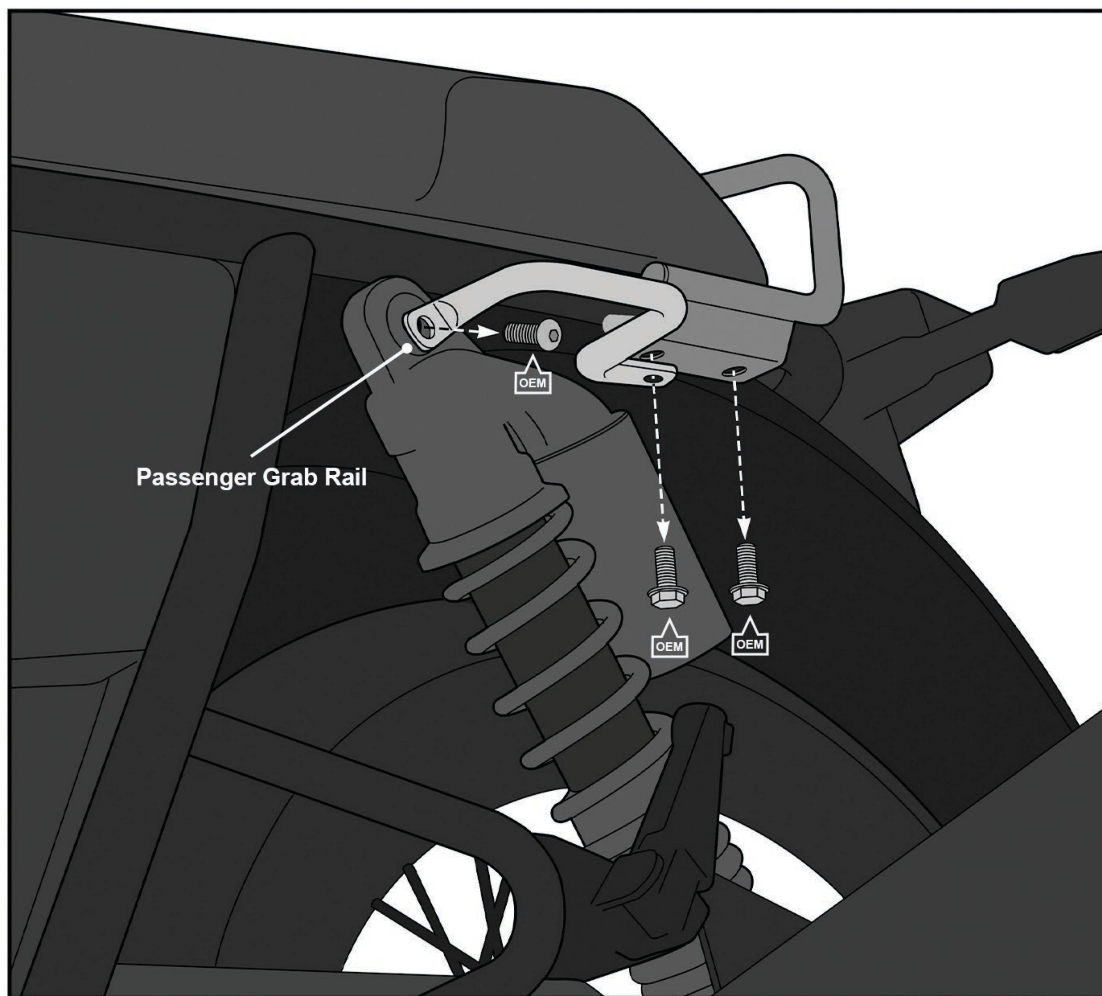
Fig 1. Remove OEM bolts and passenger grip
