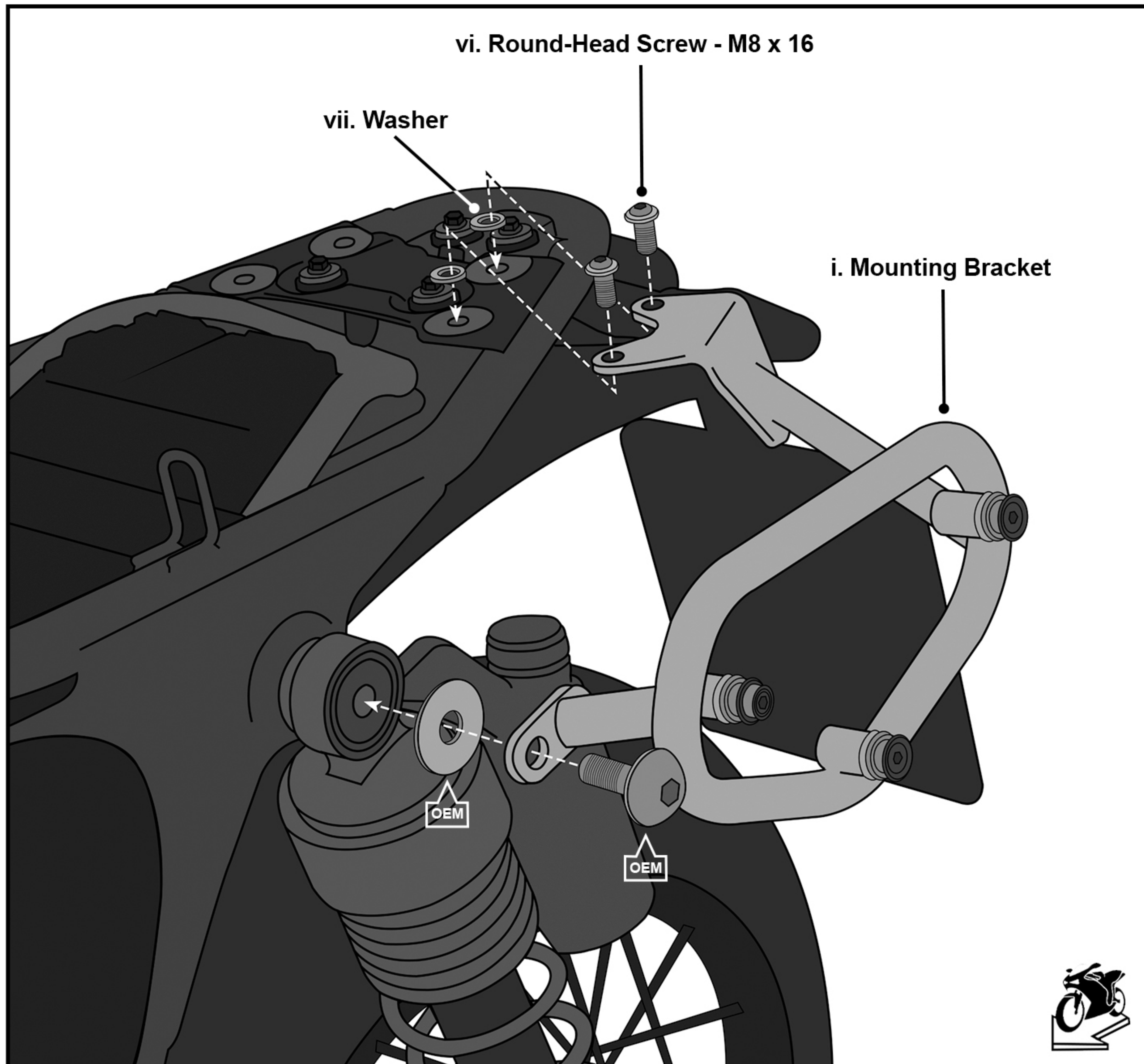
Fig 2. Installing the Mounting Bracket
