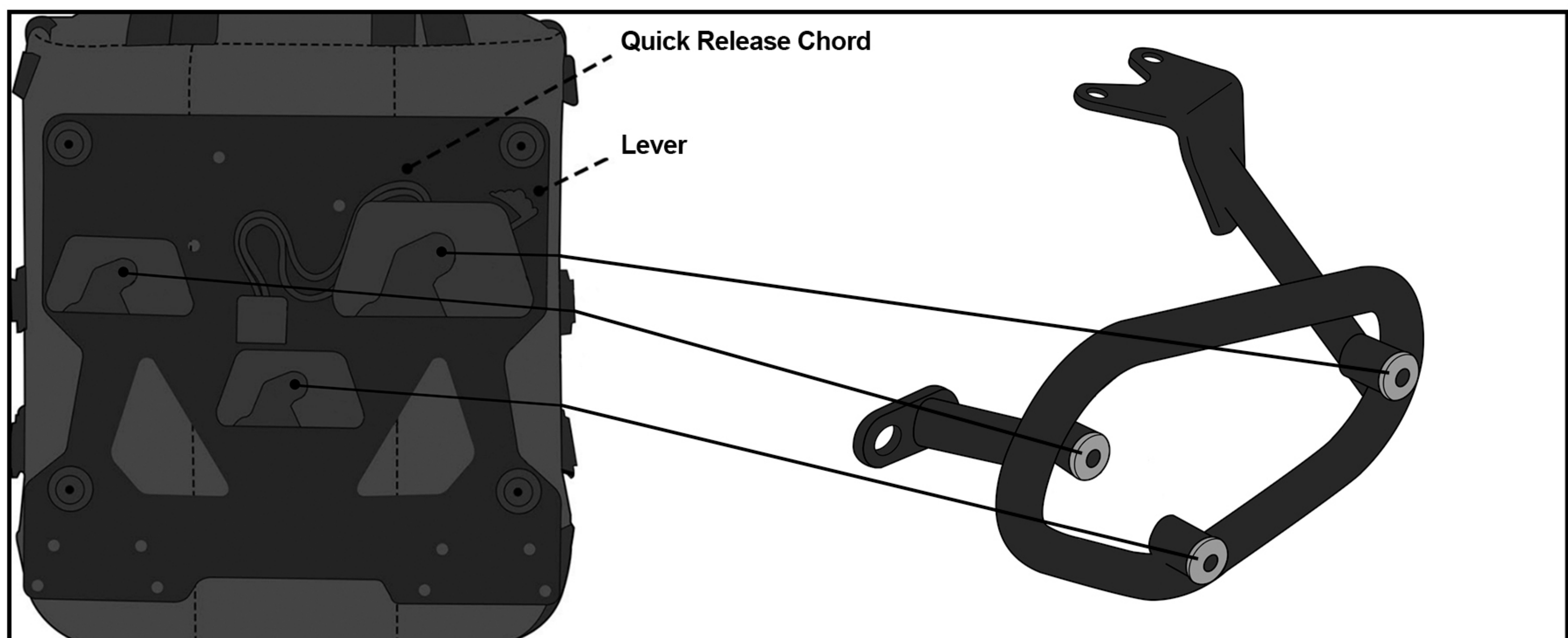
Fig 4. Attaching the Saddlebag
