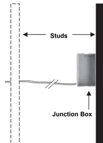
Figure 2. Junction Box Installation.
