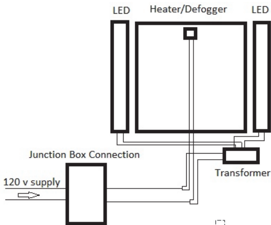
Figure 1. ClearLite Wiring Diagram.
