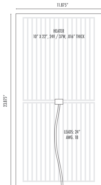
BACK VIEW SCALE 3"=1'-0"
