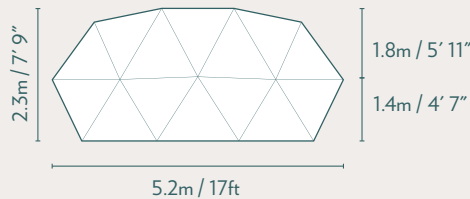
CLEAR VIEW STRUCTURE WINDOWS With Cover On
