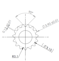
15T 4mm Output Shaft Spline
