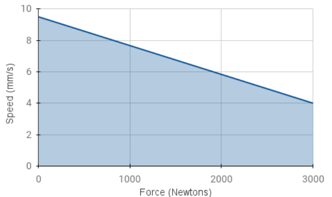
GLA3000-N 12V Force vs. Speed
