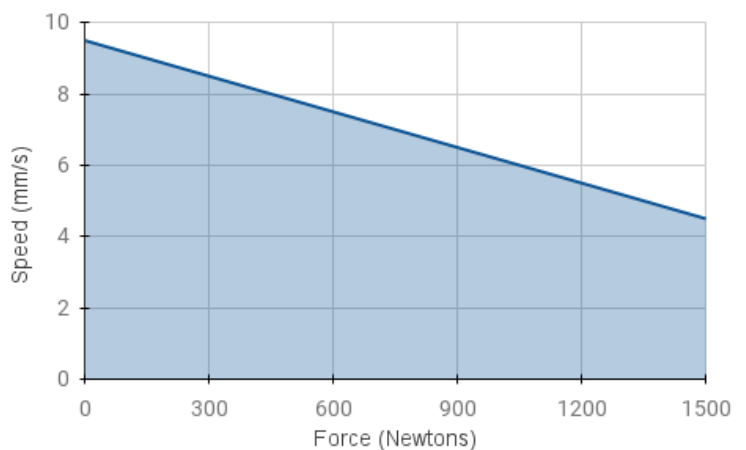
GLA1500-N Force vs. Speed (at 12V DC)
