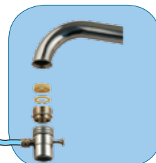
Female Tap Fitting
