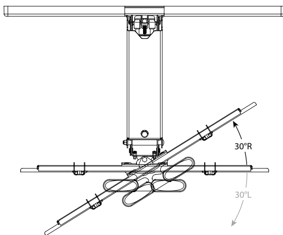
Overhead View
