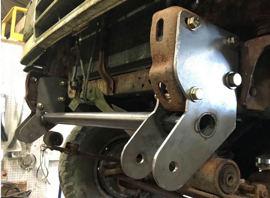
frame bracket.
