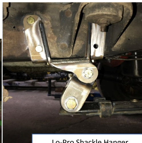
Lo-Pro Shackle Hanger
