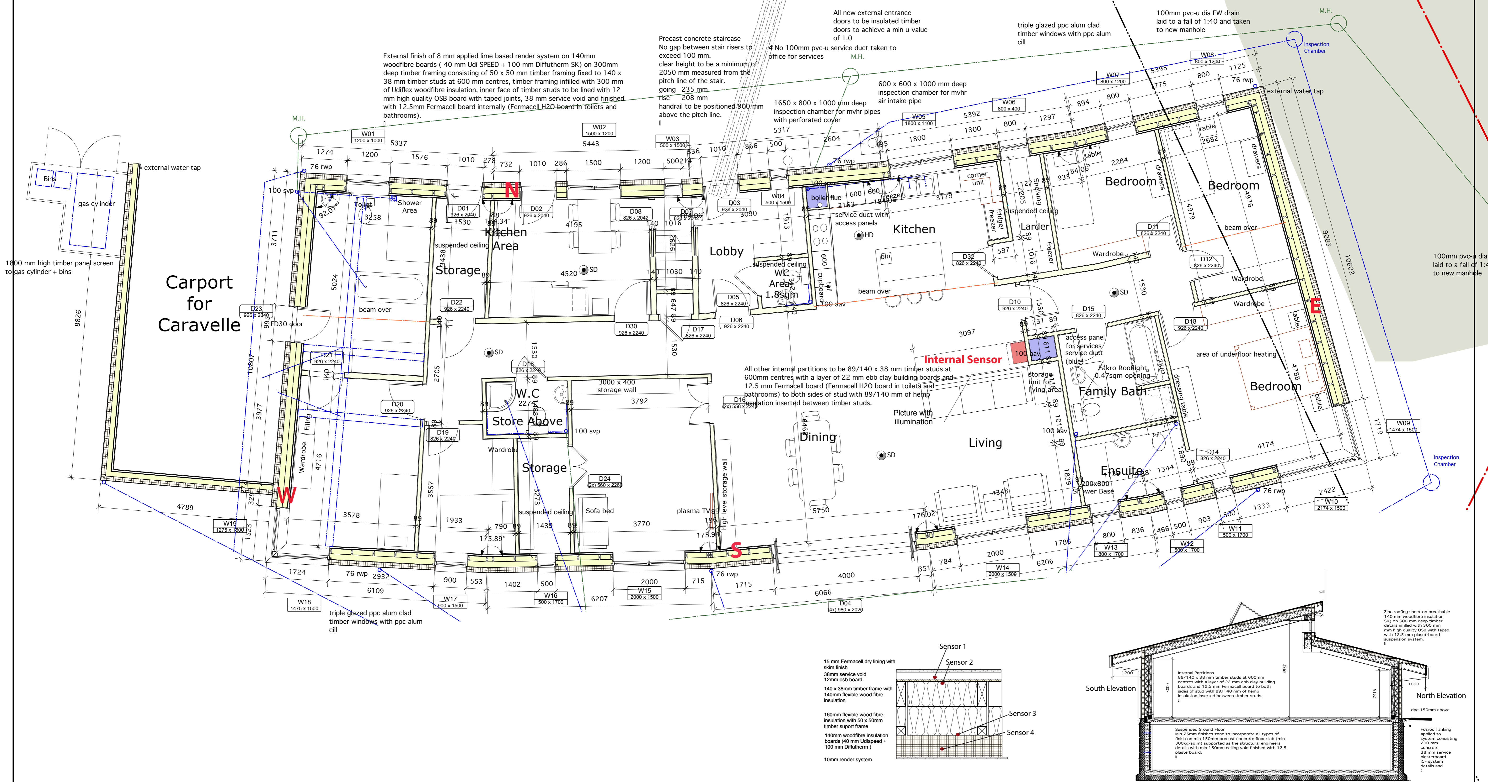
Typical External Wall Detail 1:10
