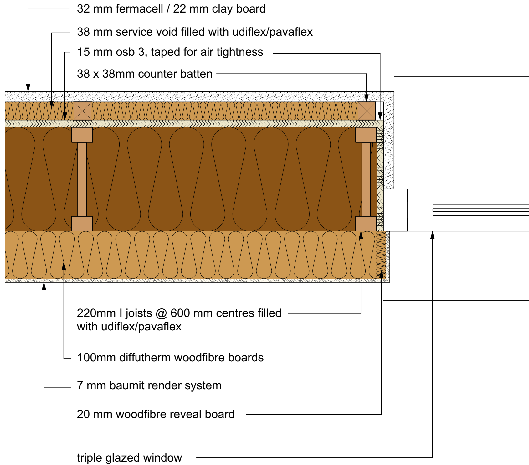
Rendered window reveal in plan
