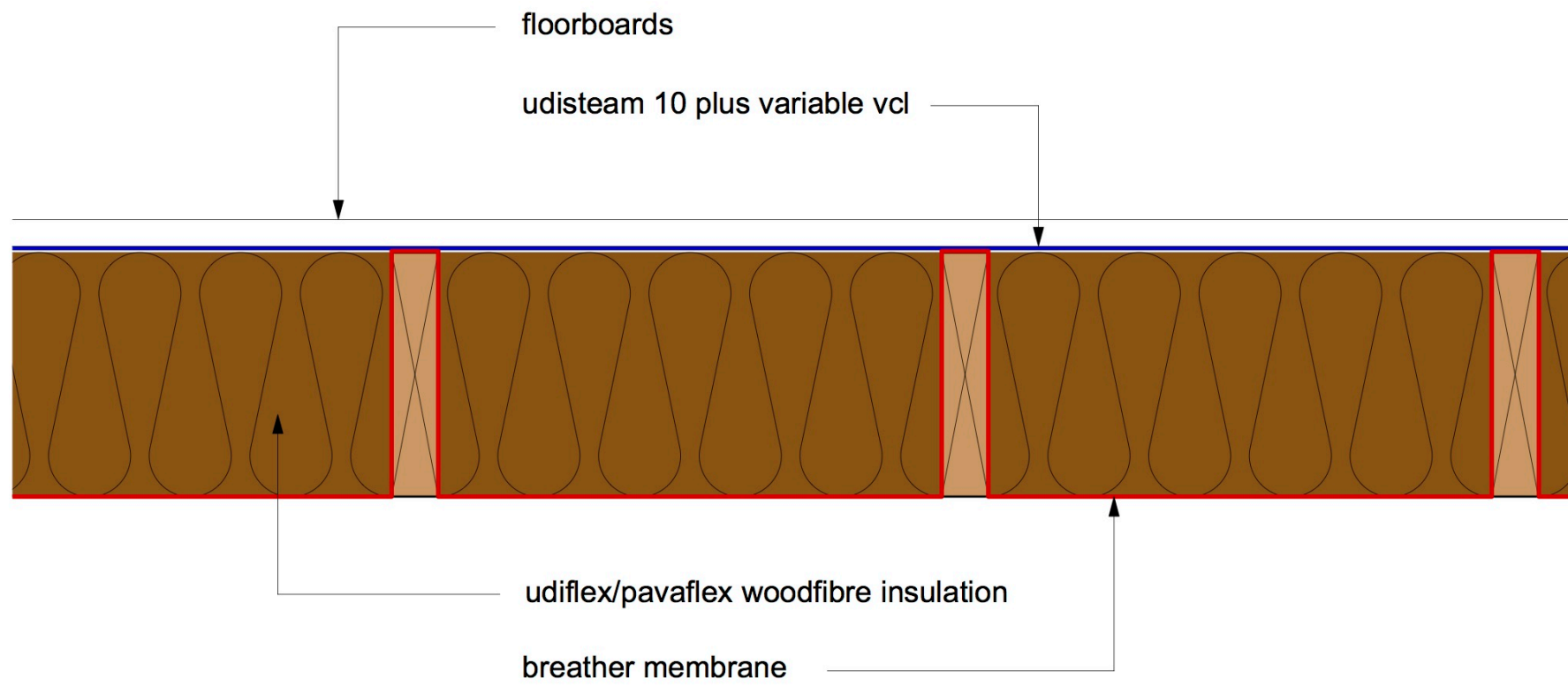
Suspended floor insulation installed from above
