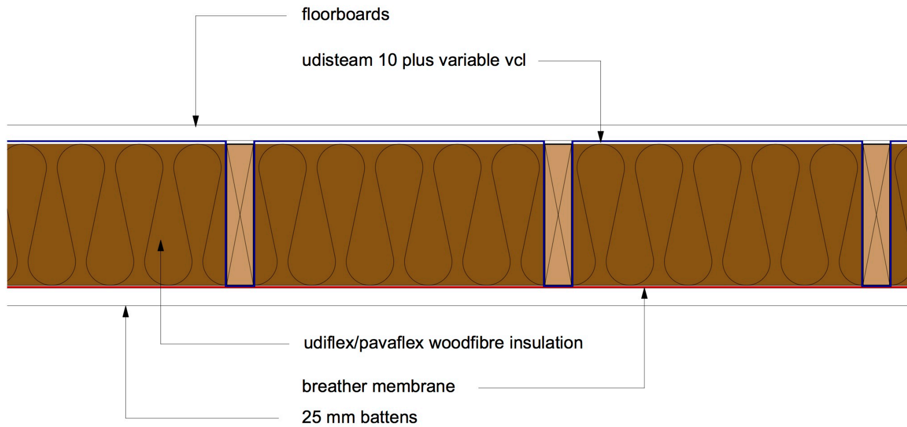
Suspended floor insulation installed from below
