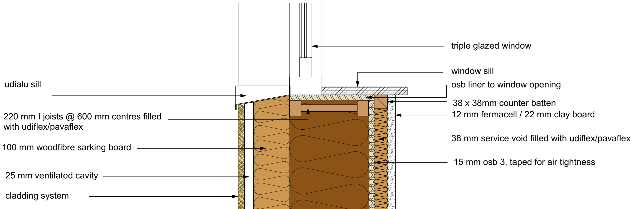
Clad window details
