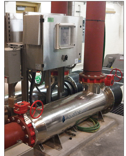
The highly efficient “L-shaped” design and low-pressure, high-output (LPHO) amalgam lamps result in an extremely compact footprint.
