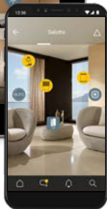
"Personalise" screen.
