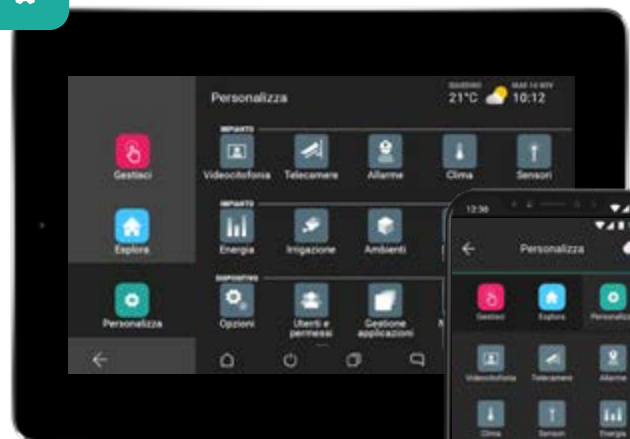
"Personalise" screen.
