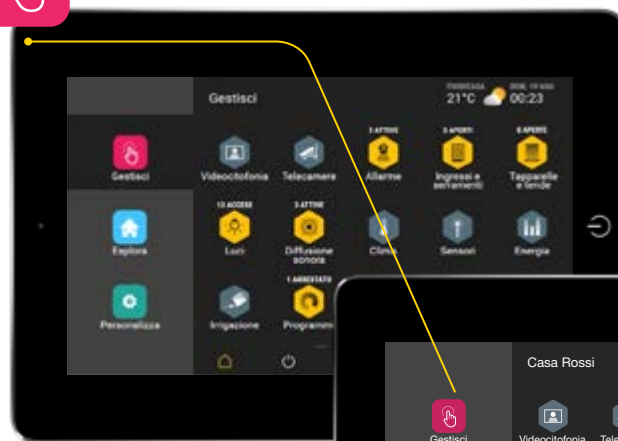
"Manage" screen
