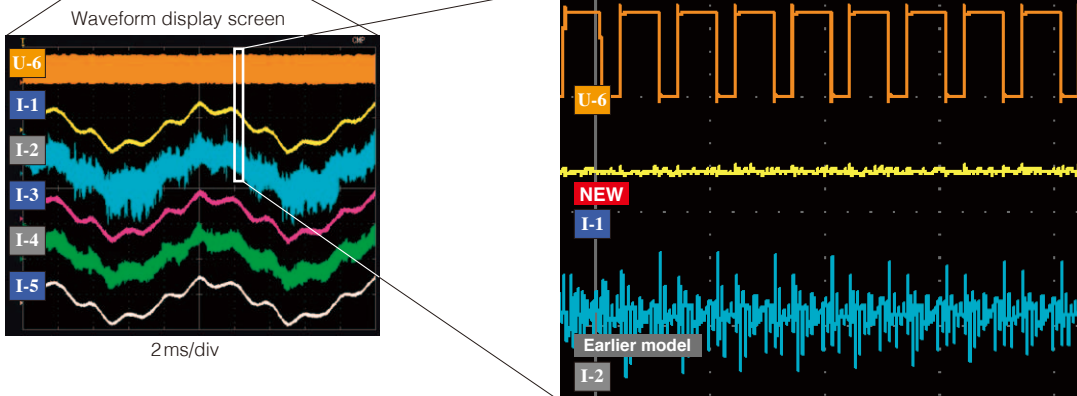
CT687x current sensors can accurately measure currents that were hidden by noise when observed with earlier models because they are not affected by noise that accompanies switching at a high carrier frequency (FSW: 100 kHz).
