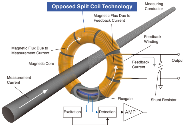
*Opposed Split Coil: Coil in which divided windings are arranged opposite each other on a magnetic core to broaden the range of current detection
