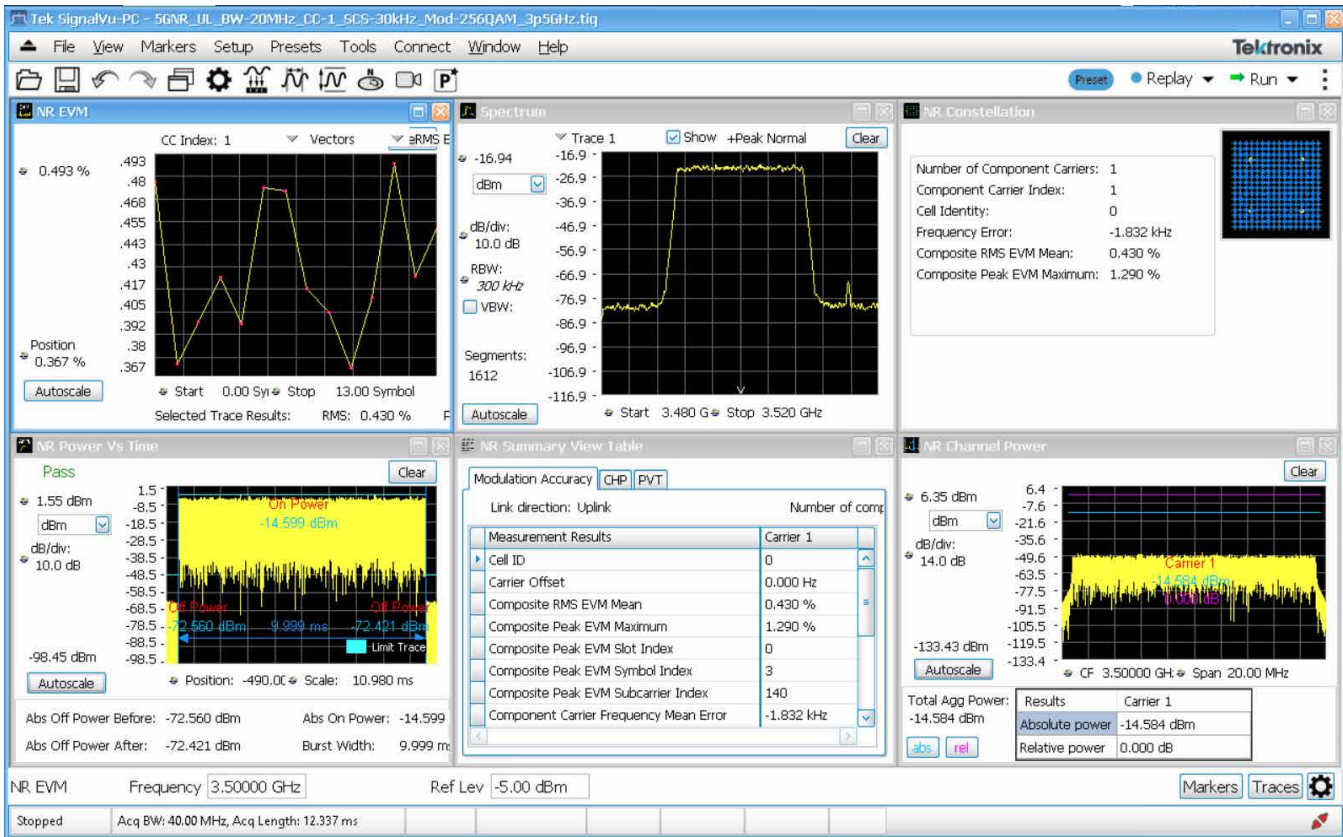
Constellation, Summary View, EVM, EVM vs, Symbol, Frequency error, PVT, and CHP displays supported in option 5G NR
