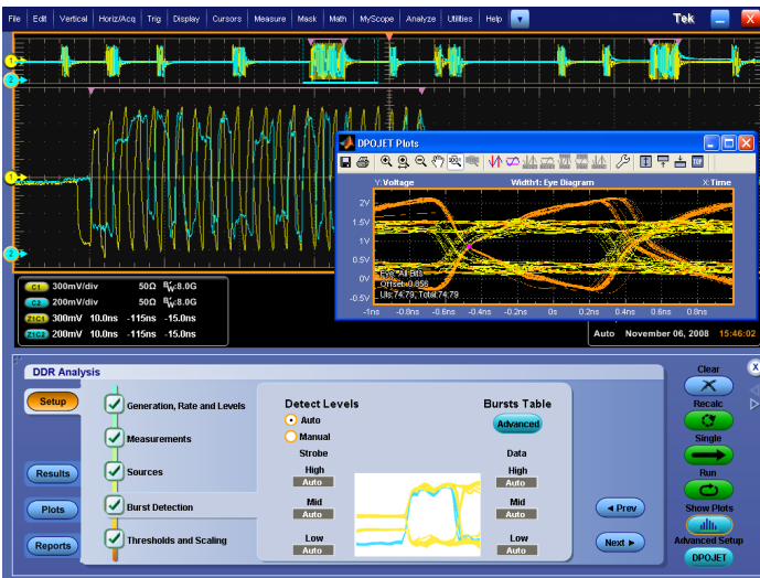
DDR Memory Bus Analysis (Option DDRA) – Automatically identifies DDR1, LPDDR, LPDDR2, LPDDR3, DDR2, DDR3, DDR4, and GDDR3 Reads and Writes and makes JEDEC conformance measurements with pass/fail results on all edges in every Read and Write burst. DDRA provides capabilities for measurements of clock, address, and control signals. In addition to enabling conformance testing DDRA with DPOJET is the fastest way to debug complex memory signaling issues.
