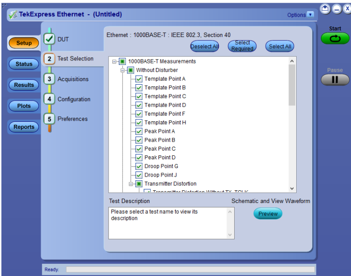
Ethernet Compliance Test Solution (Option ET3) – Receive full PHY layer support for Ethernet variants 10BASE-T, 100BASE-TX, and 1000BASE-T with the comprehensive, integrated Tektronix® Ethernet tool set. Analog verification, automated compliance software, and device characterization solutions are all included.
