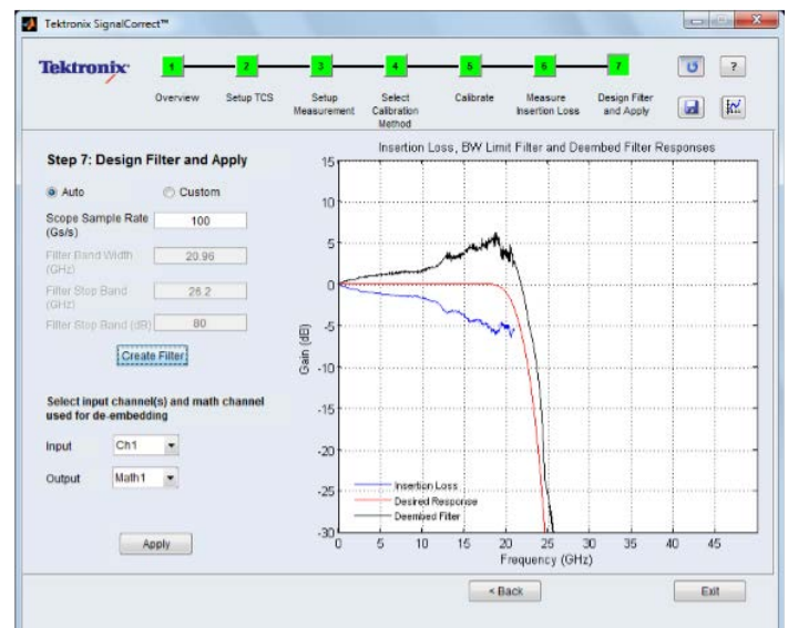
SignalCorrect creates a filter that you can apply to your oscilloscope inputs to de-embed your device or interconnect under test.
