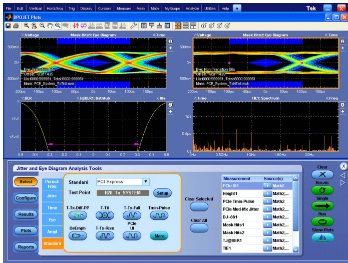
PCI Express® Transmitter Compliance and Debug (Option PCE3 and PCE4) – Analyze the performance of your PCI Express® Gen 1, 2, 3, or 4 design with comprehensive test support. Using DPOJET, Option PCE3 and PCE4 enable tests that conform to PCI-SIG standards.
