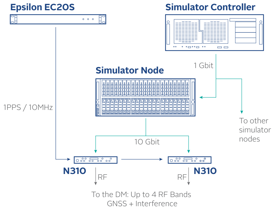
Figure 6 – Simulator node
