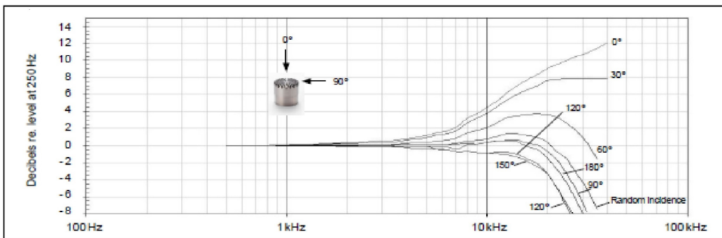
Free-field corrections for various degrees of incidence
