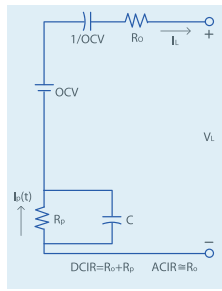
Li-ion battery Equivalent Circuit Model
