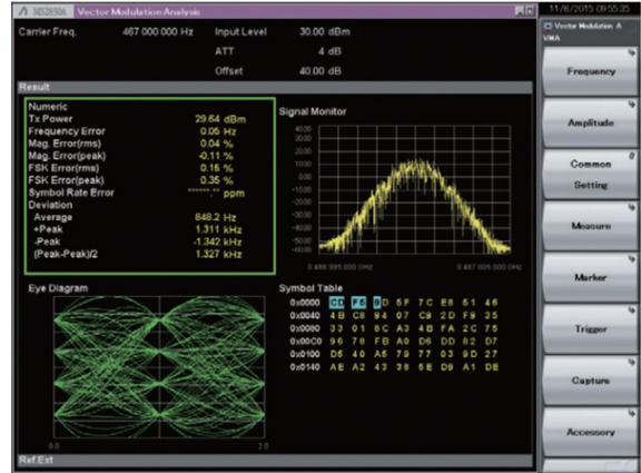
4FSK Modulation Analysis Measurement Example
