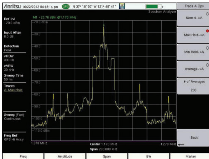
AM broadcast profiling
