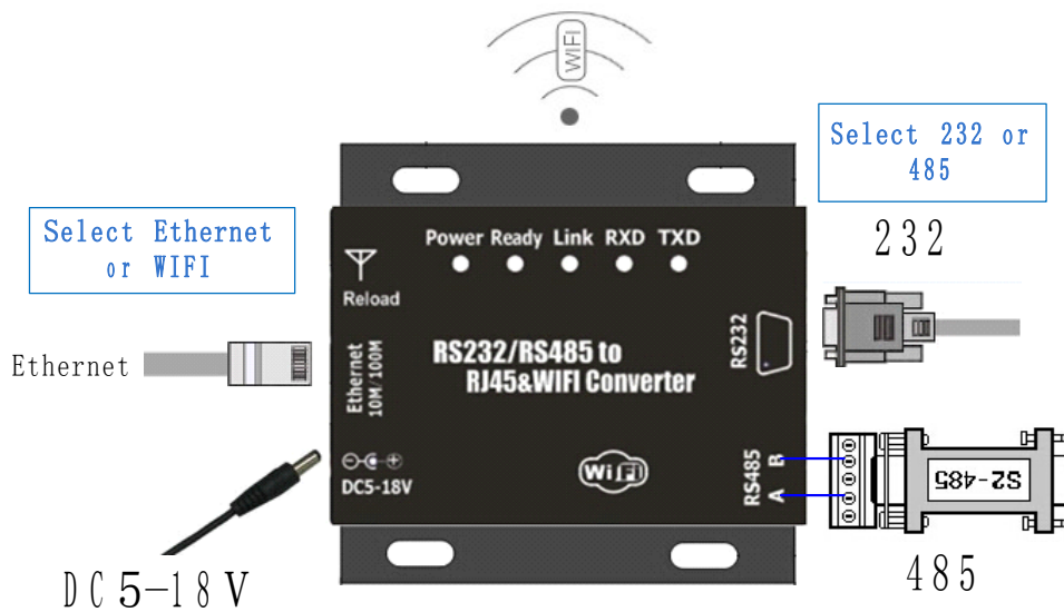
Figure 1 Hardware Connect(610)
