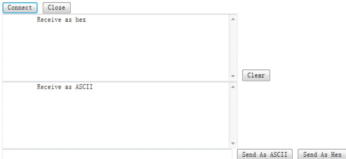
Figure 9 Websocket Page
